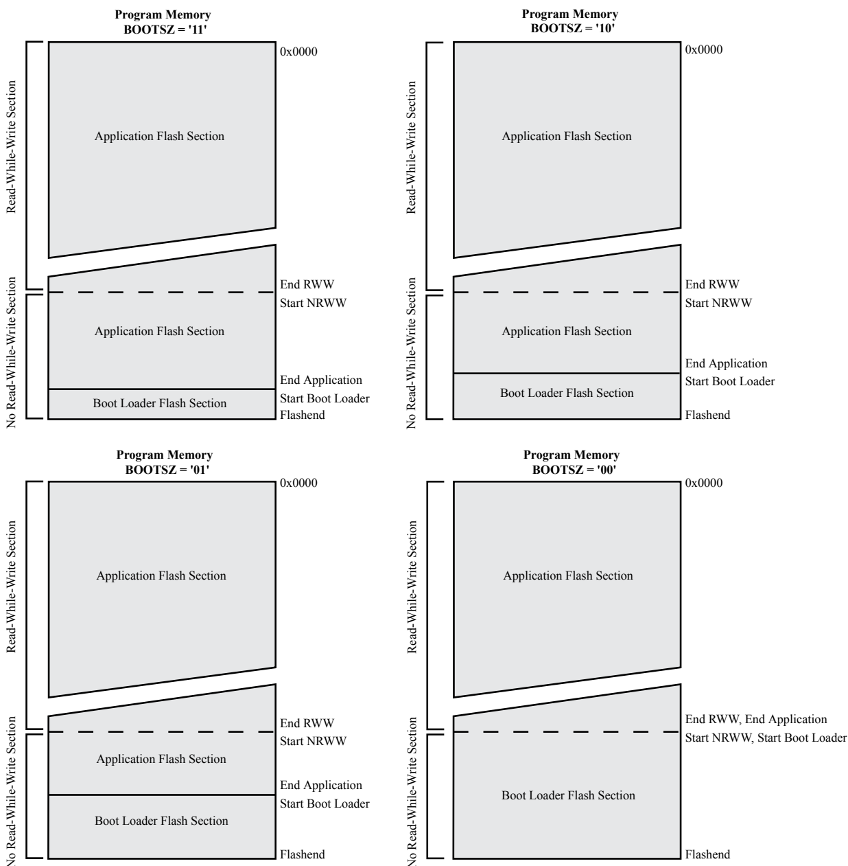
Figure 31-2. Memory Sections
