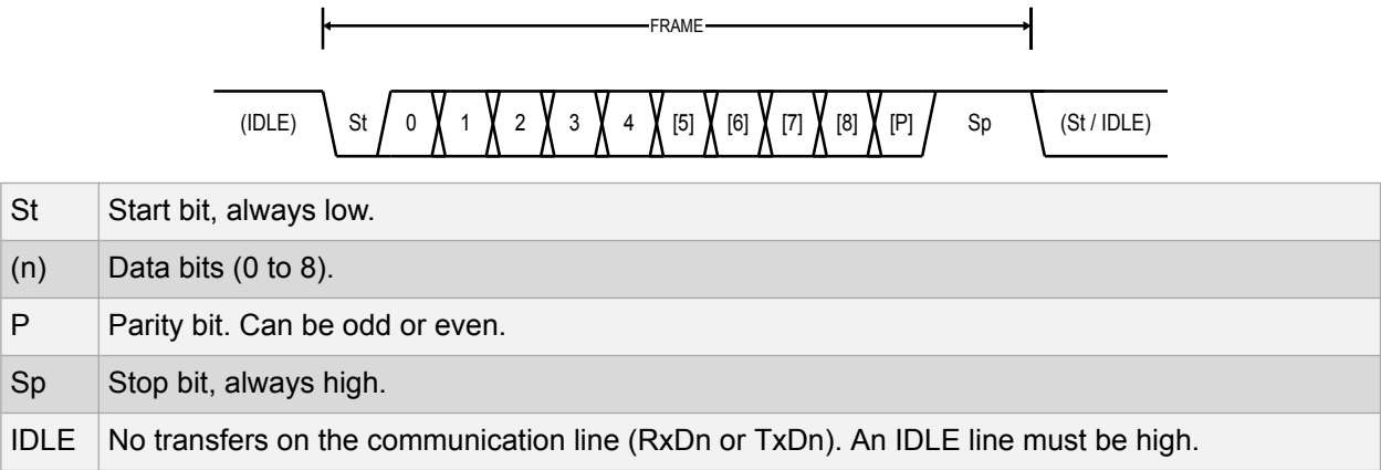
Figure 24-4. Frame Formats
