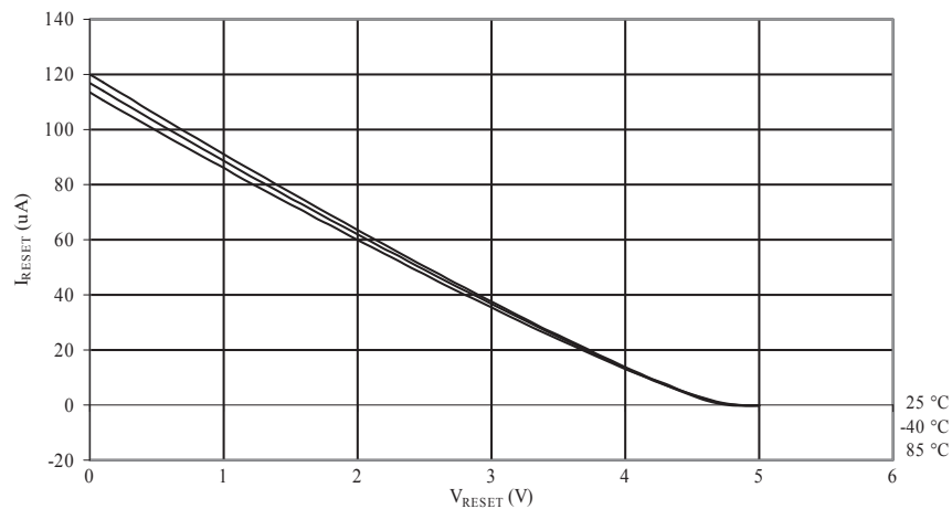
Figure 34-20. ATmega48P/PV: Reset Pull-up Resistor Current vs. Reset Pin Voltage ( V_{CC} = 5V )
