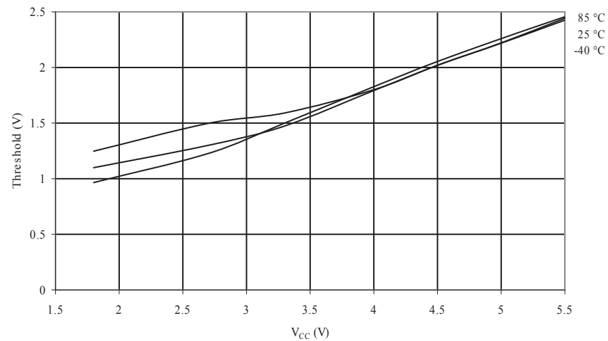
Figure 34-29. ATmega48P/PV: Reset Input Threshold Voltage vs. V_{CC} ( V_{IL} , I/O Pin read as '0')
