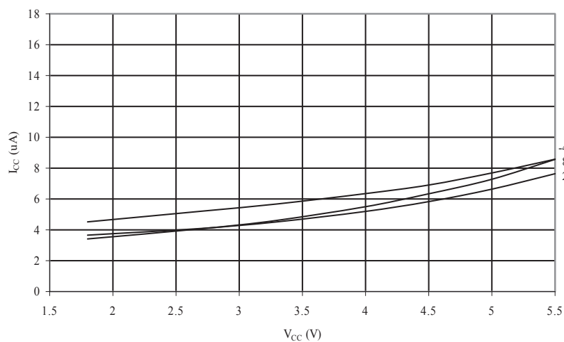
Figure 34-12. ATmega48P/PV: Power-Down Supply Current vs. V_{CC} (Watchdog Timer Enabled)
