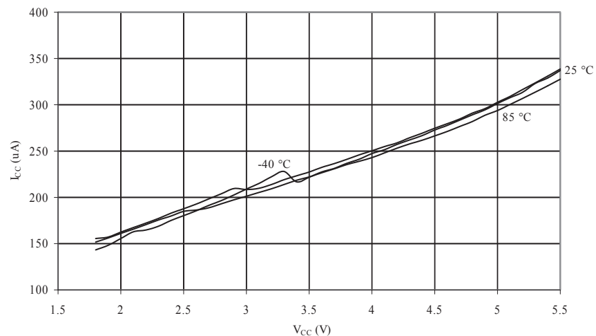
Figure 34-131. ATmega168P/PV: ADC Current vs. V_{CC} (AREF = AV_{CC} )
