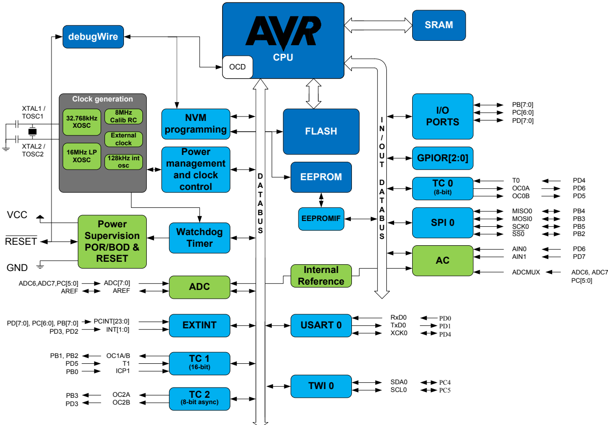
Figure 4-1. Block Diagram
