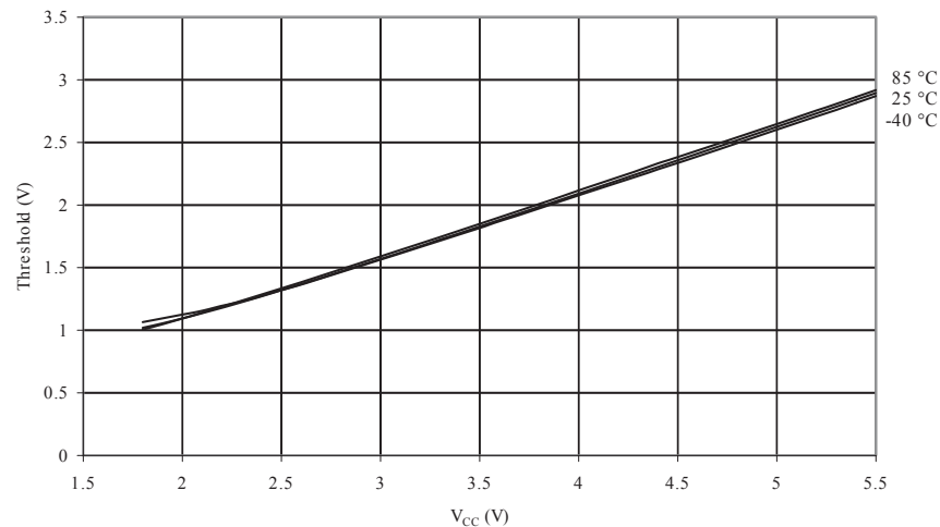
Figure 34-117. ATmega168P/PV: I/O Pin Input Threshold Voltage vs. V_{CC} ( V_{IH} , I/O Pin read as '1')
