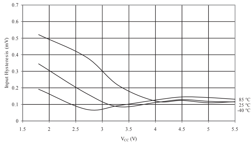
Figure 34-30. ATmega48P/PV: Reset Pin Input Hysteresis vs. V_{CC}
