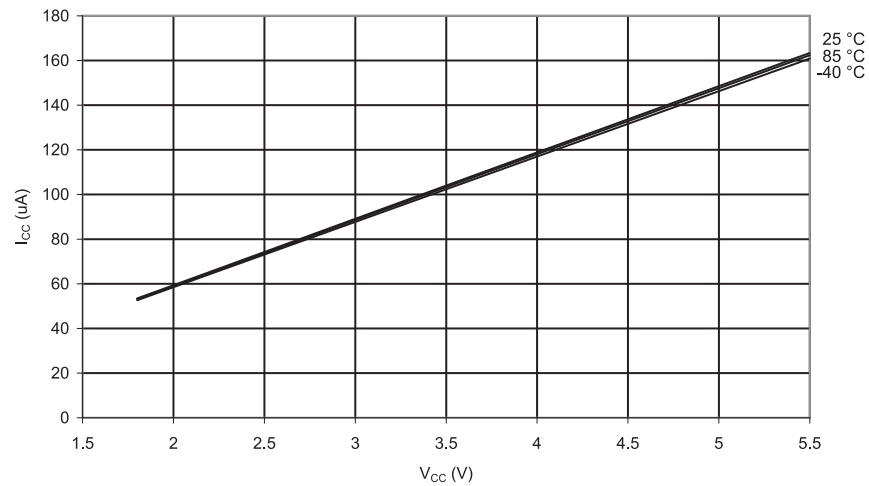
Figure 34-134. ATmega168P/PV: Brownout Detector Current vs. V_{CC}
