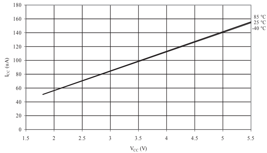
Figure 34-42. ATmega48P/PV: Brownout Detector Current vs. V_{CC}
