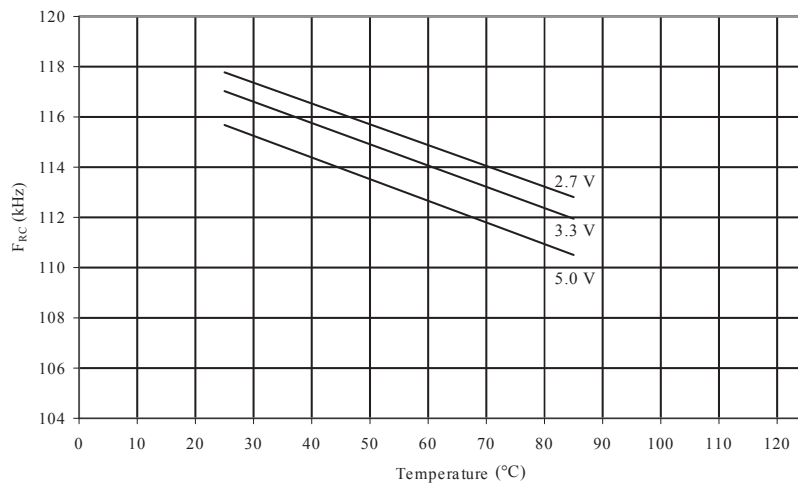
Figure 34-127. ATmega168P/PV: Watchdog Oscillator Frequency vs. V_{CC}
