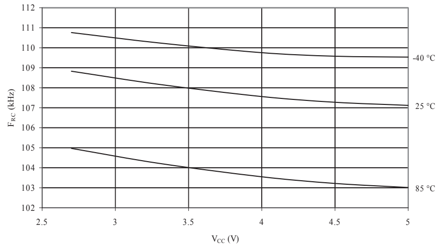
Figure 34-82. Calibrated 8 MHz RC Oscillator Frequency vs. V_{CC}
