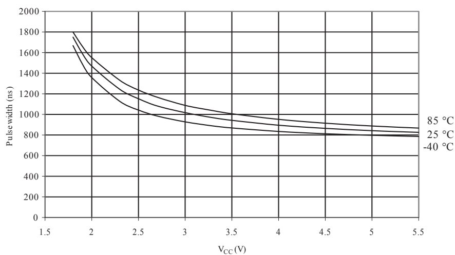
Figure 34-92. Minimum Reset Pulse Width vs. Vcc
