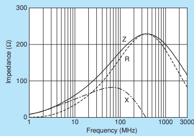
BLM18PG181SN1
