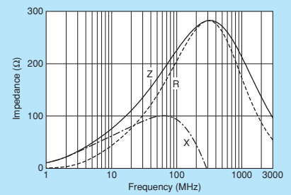
BLM18PG221SN1
