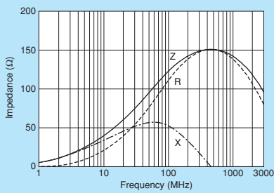
BLM18PG121SN1
