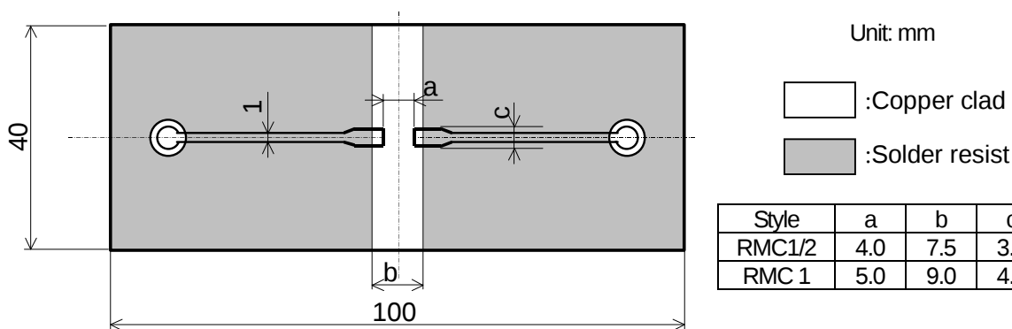
RMC1/2, 1 BOUND STRENGTH OF THE END FACE PLATING TEST SUBSTRATE
