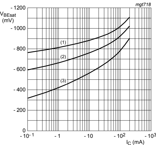
Figure 6. BC856B; BC857B; BC858B: Base-emitter voltage as a function of collector current; typical values
