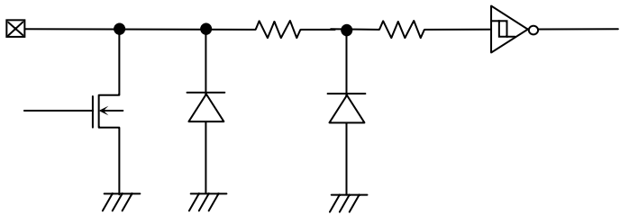
Figure 57. Input / output pin circuit diagram
