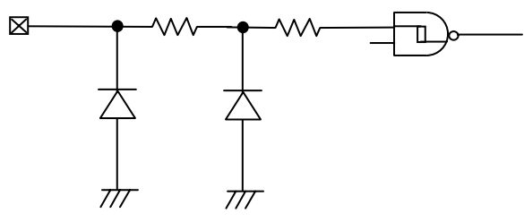
Figure 58. Input pin circuit diagram
