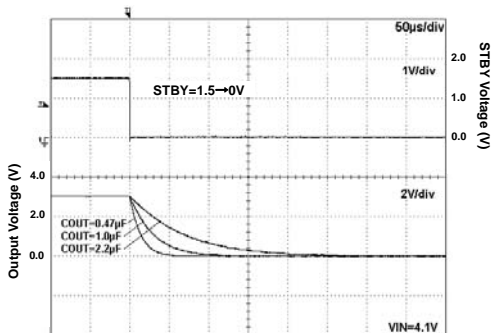
Fig 257. Discharge Time
