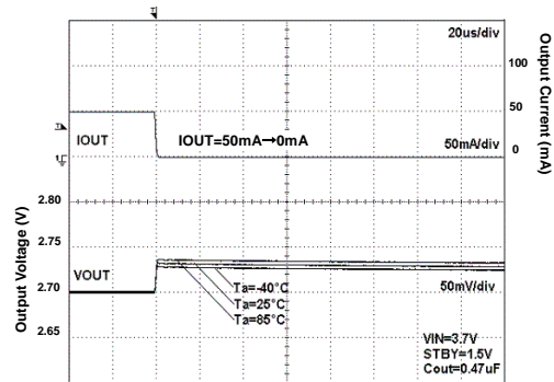
Fig 168. Load Response
