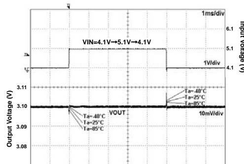
Fig 258. VIN Response
