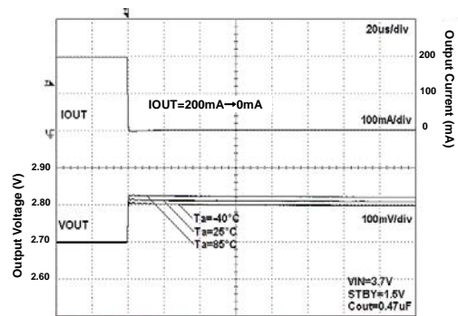
Fig 172. Load Response
