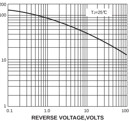
FIG. 5-TYPICAL JUNCTION CAPACITANCE
