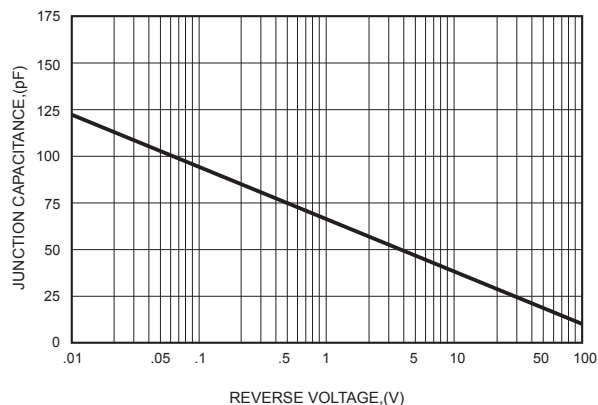
FIG.6-TYPICAL JUNCTION CAPACITANCE
