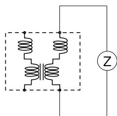
(C)差模
