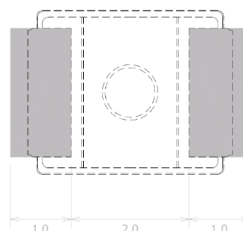
Figure 1. IN-P32ZTIR Solder Pattern
