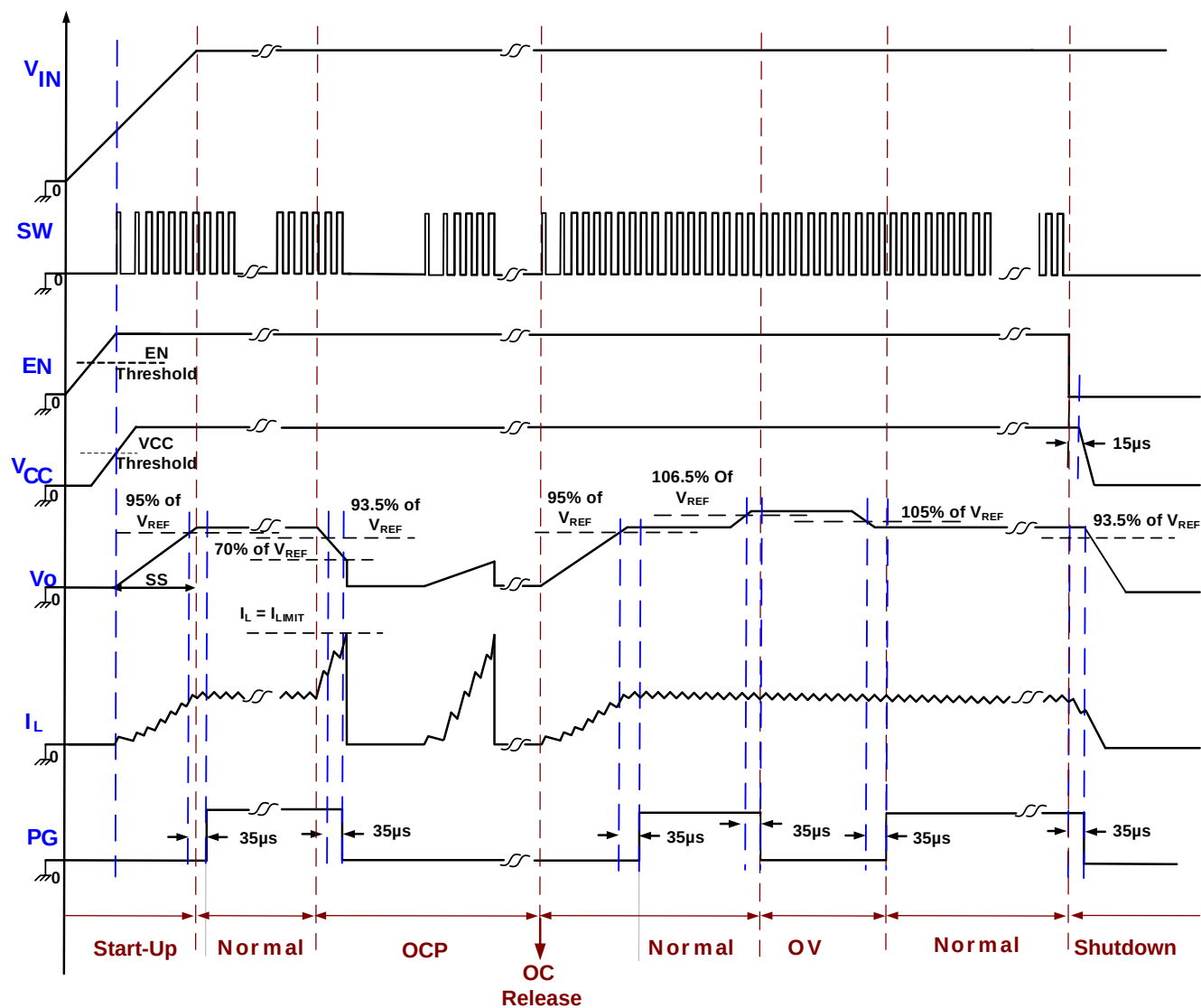
Figure 5: Timing Sequence
