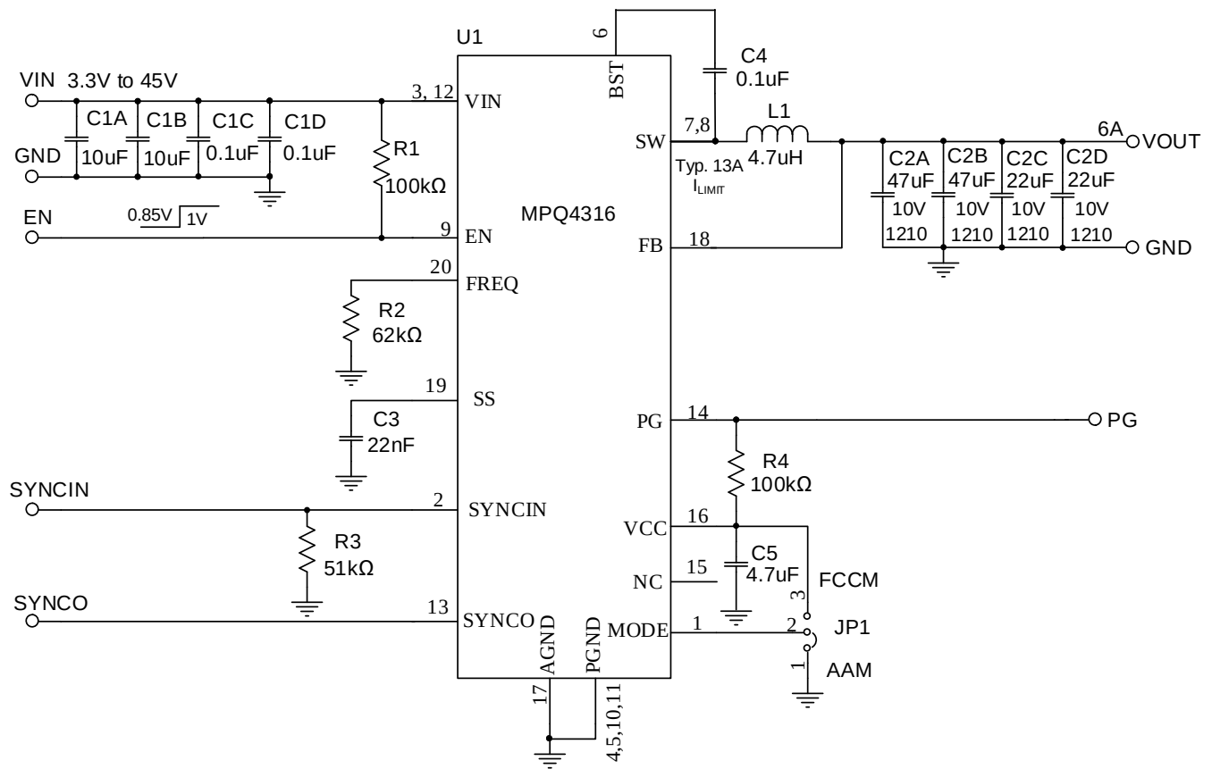
Figure 15: f_{sw} = 470\text{kHz} , Fixed Output
