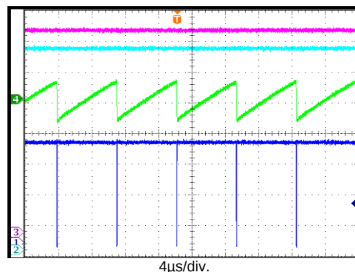
Dropout Operation
