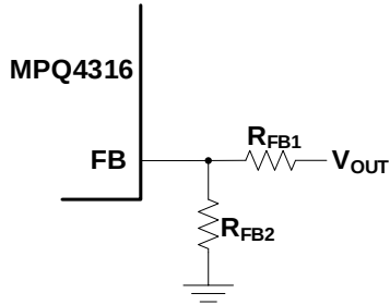
Figure 9: Feedback Network
