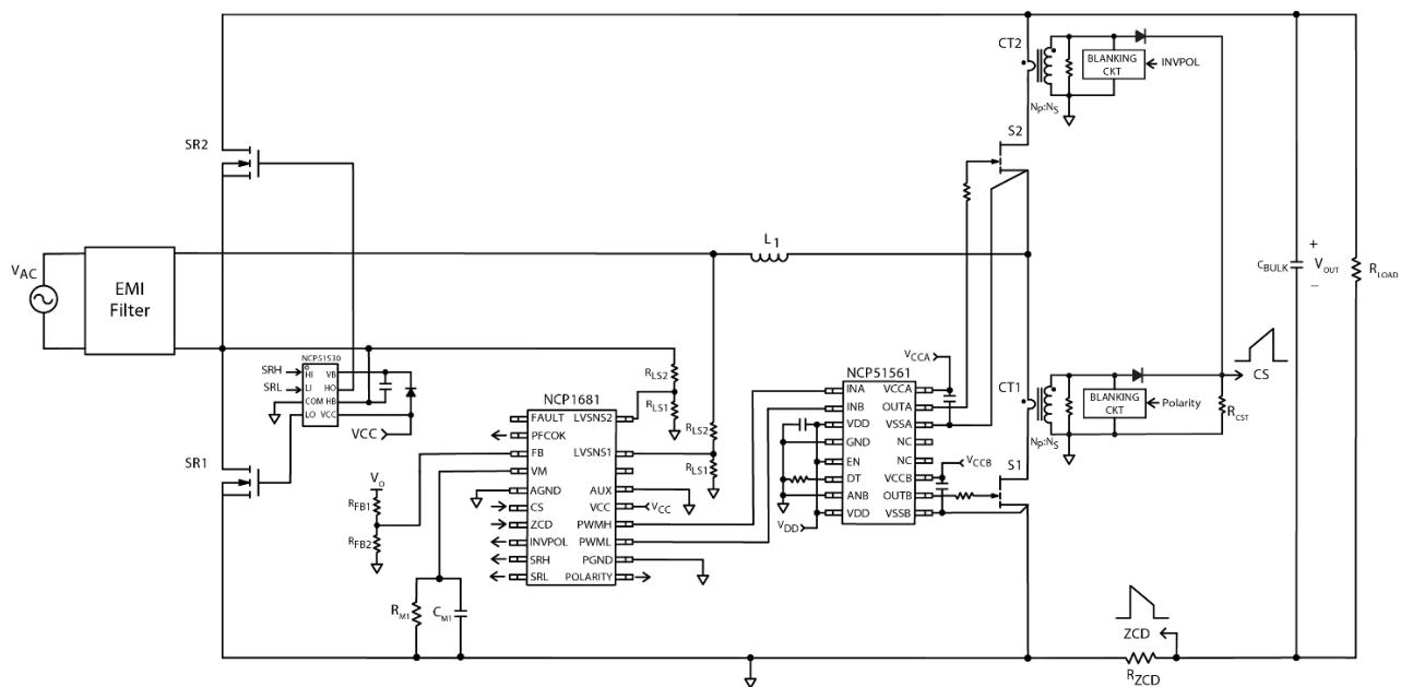
Figure 1. Typical CCM Application Schematic
