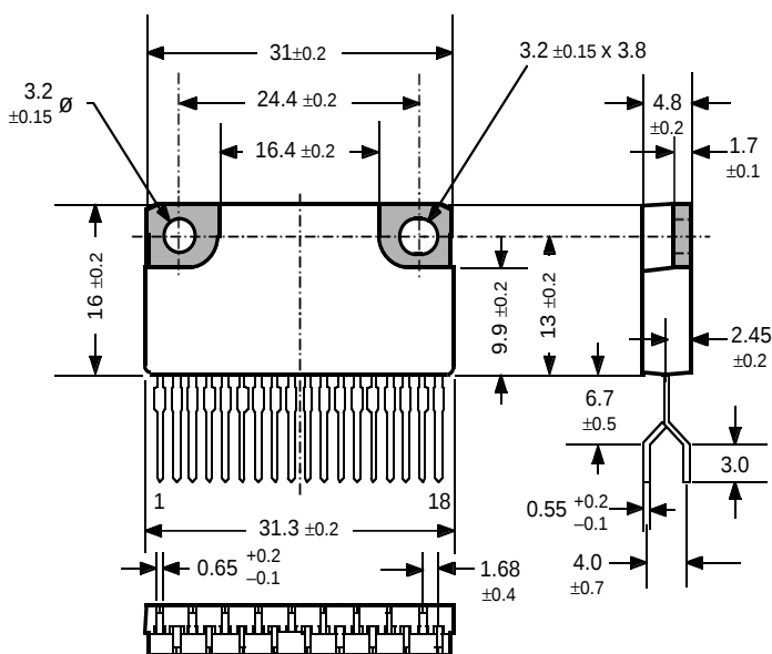
Dimensions in Millimeters (controlling dimensions)
