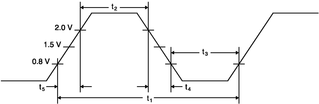
Figure 39. CLK Waveforms
