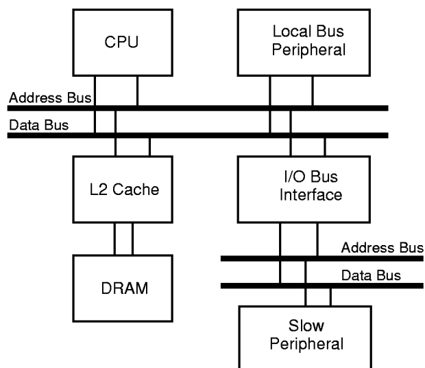
Figure 3. Typical System Block Diagram for \text{HOLD}/\overline{\text{HLDA}} Bus Arbitration
