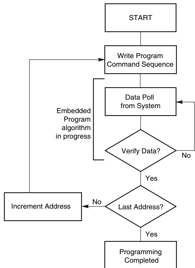
Figure 1. Program Operation
