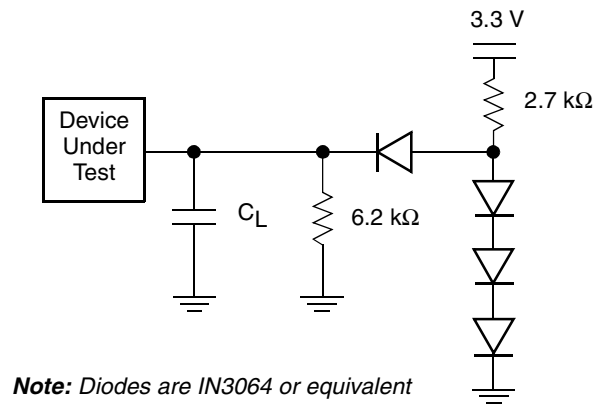
Figure 9. Test Setup
