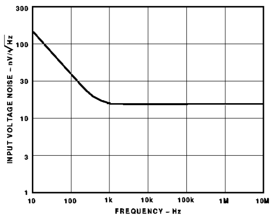
Figure 10. Input Voltage Noise vs. Frequency
