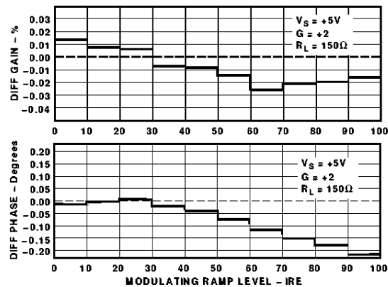
Figure 13. Differential Gain and Phase Errors
