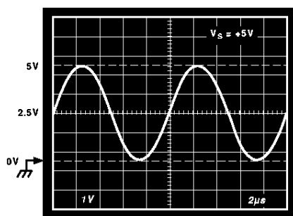
Figure 1. Output Swing: Gain = -1, R_L = 2 \text{ k}\Omega
