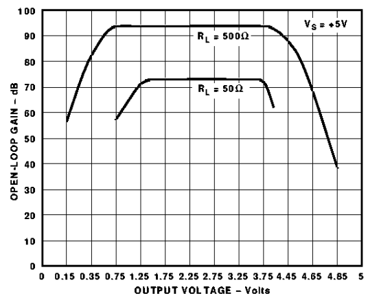
Figure 9. Open-Loop Gain vs. Output Voltage
