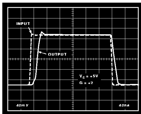
Figure 33. Overdrive Recovery
