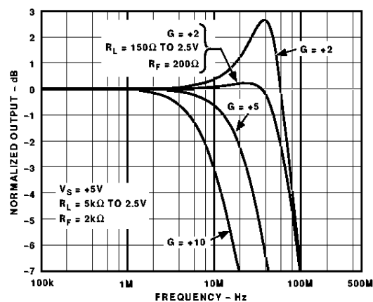
Figure 26. Frequency Response vs. Closed-Loop Gain
