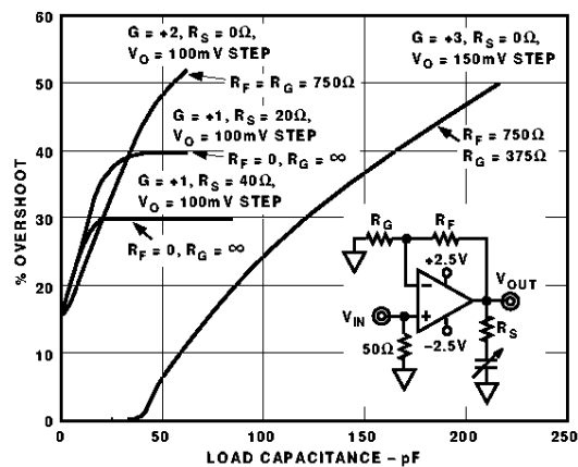
Figure 25. % Overshoot vs. Capacitive Load
