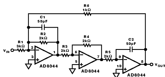
Figure 38. 2 MHz Biquad Bandpass Filter Using AD8044
