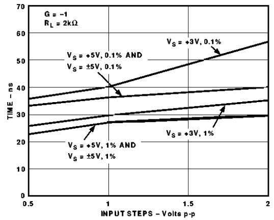
Figure 19. Settling Time vs. Input Step
