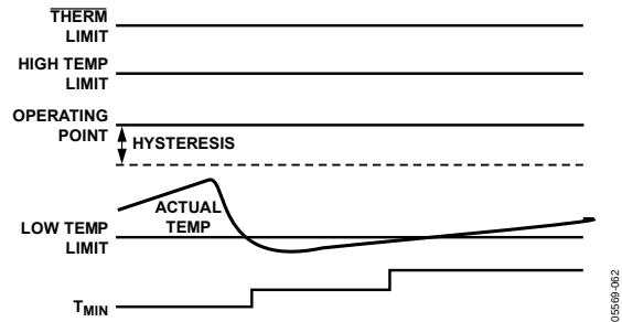
Figure 73. Increasing T_{MIN} for Quieter Operation
