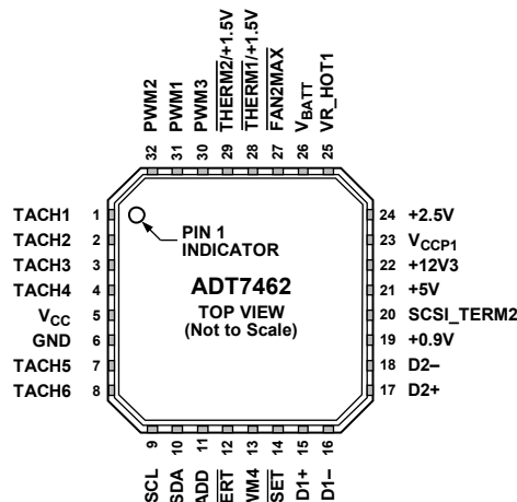
Figure 7. Configuration Option 4
