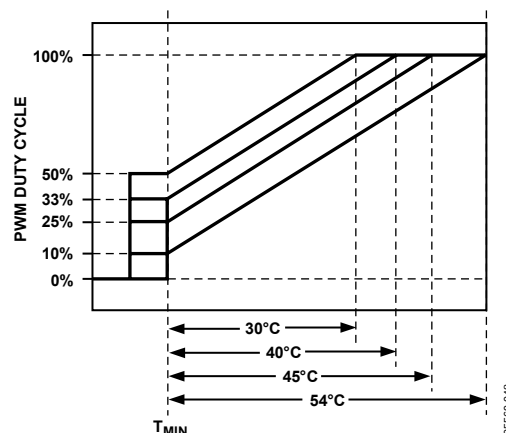
Figure 60. Increasing PWM MIN Changes Effective T RANGE
