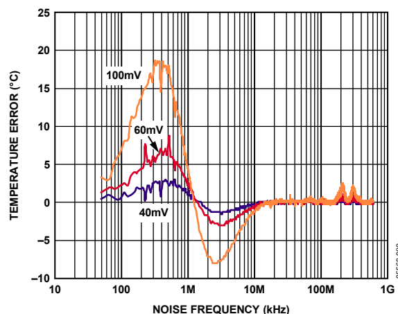
Figure 18. Remote Temperature Error vs. Common-Mode Noise Frequency
