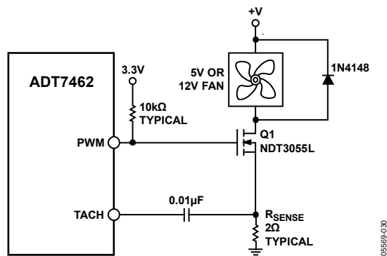
Figure 40. Driving a 2-Wire Fan
