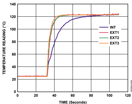
Figure 14. ADT7462 Response to Thermal Shock
