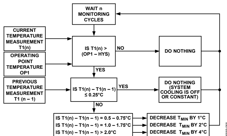
Figure 69. Short Cycle Steps
