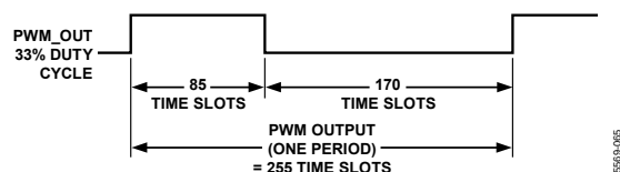
Figure 76. 33% PWM Duty Cycle Represented in Time Slots
