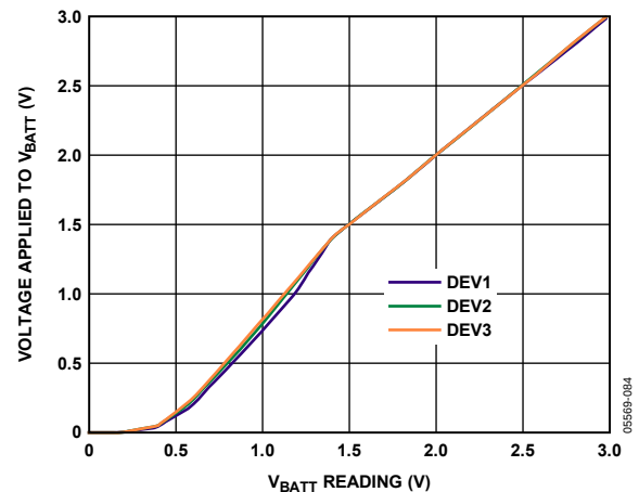
Figure 22. Applied Voltage vs. V_{BATT} Reading
