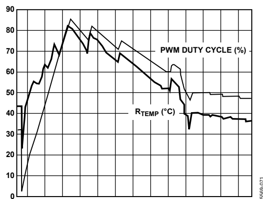
Figure 82. How Fan Reacts to Temperature Variations in Enhanced Acoustics Mode
