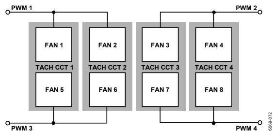
Figure 83. Fan Freewheeling Test Mode Setup
