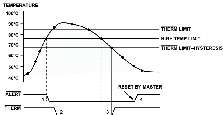
Figure 84. \overline{\text{THERM}} Behavior
