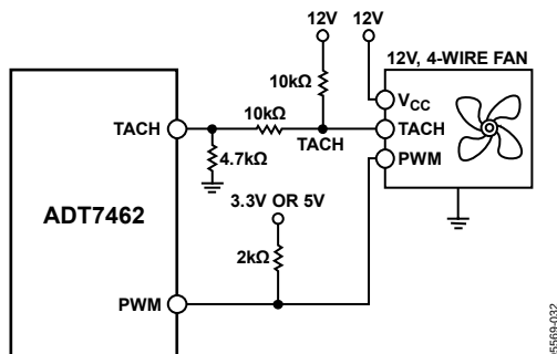
Figure 42. Driving a 4-Wire Fan
