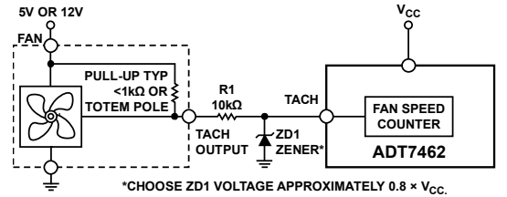
Figure 46. Fan with Strong TACH Pull-Up to > V_{CC} or Totem-Pole Output, Clamped with a Zener Diode and Resistor
