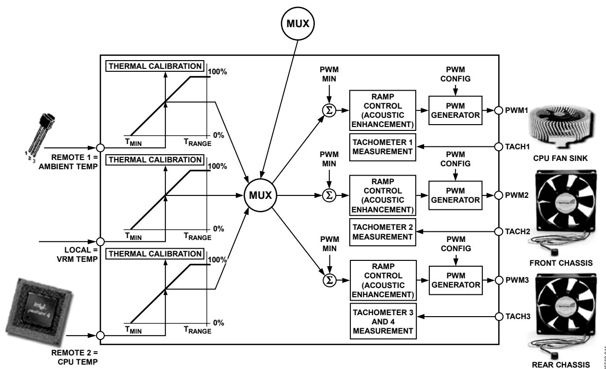
Figure 53. Assigning Temperature Channels to Fan Channels
