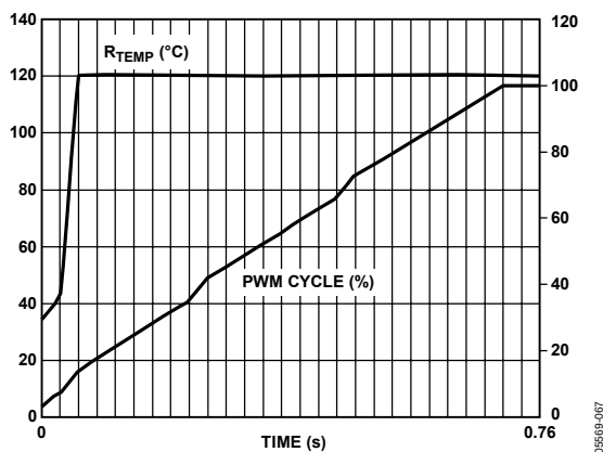
Figure 78. Enhanced Acoustics Mode with Ramp Rate = 48
