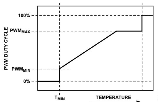
Figure 57. PWM MAX Determines Maximum PWM Duty Cycle Below the THERM Temperature Limit
