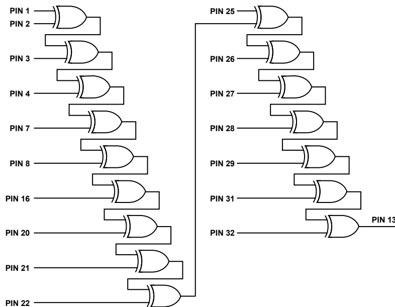
Figure 87. XOR Tree Test
