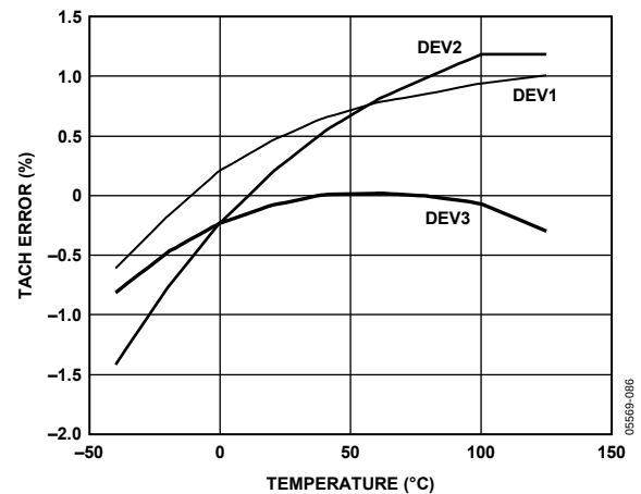
Figure 24. TACH Accuracy vs. Temperature
