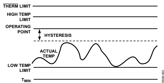
Figure 71. Temperature Between the Operating Point and the Low Temperature Limit
