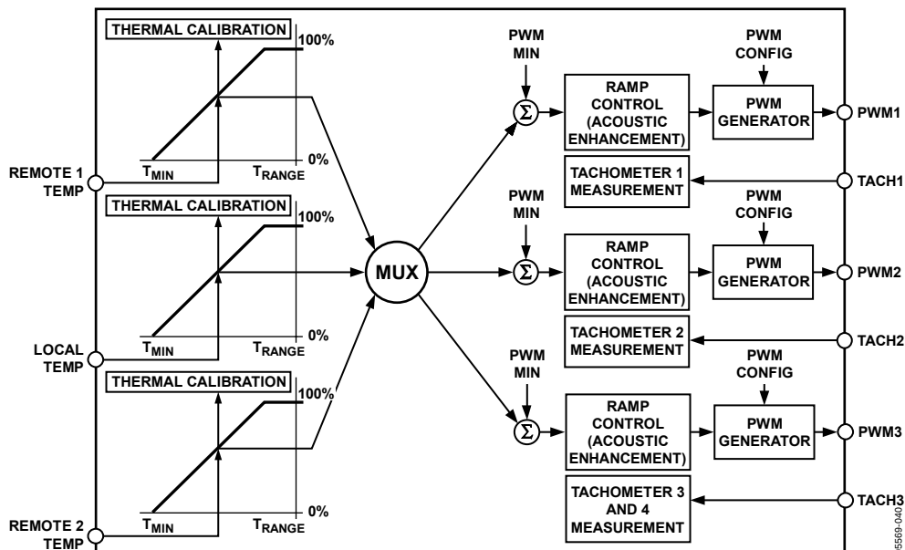
Figure 52. Automatic Fan Control Block Diagram
