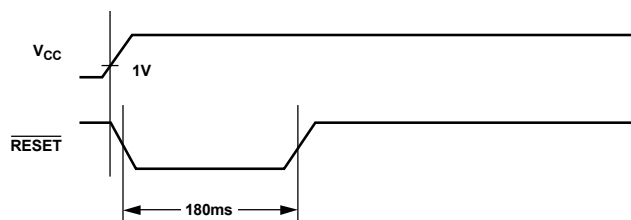
Figure 86. Operation of RESET Output on Power-Up
