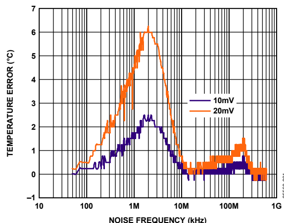
Figure 19. Remote Temperature Error vs. Differential-Mode Noise Frequency
