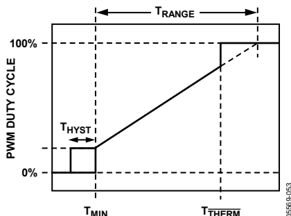
Figure 65. T_{HYST} Value Applies to Fan On/Off Hysteresis
