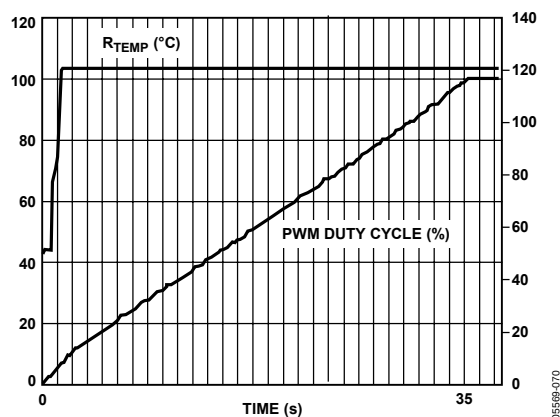
Figure 81. Enhanced Acoustics Mode with Ramp Rate = 1
