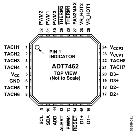
Figure 5. Configuration Option 2
