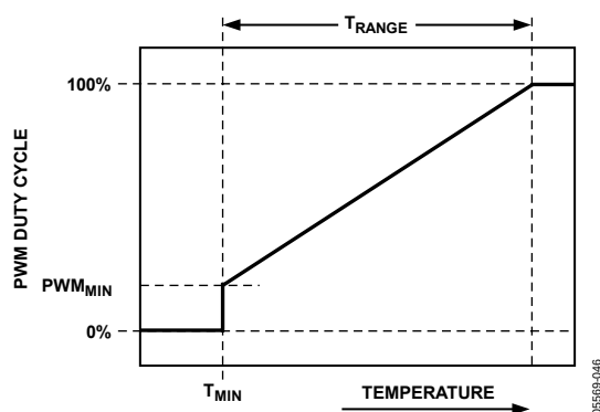
Figure 58. T RANGE Parameter Affects Cooling Range
