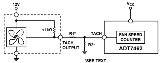
Figure 47. Fan with Strong TACH Pull-Up to > V_{CC} or Totem-Pole Output, Attenuated with R_1/R_2
