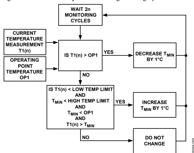
Figure 70. Long Cycle Steps
