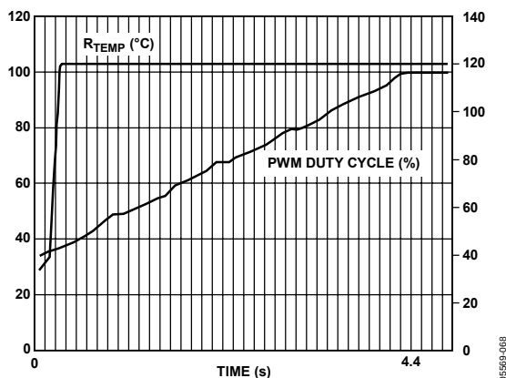
Figure 79. Enhanced Acoustics Mode with Ramp Rate = 8
