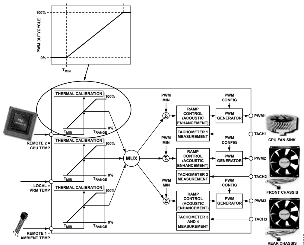
Figure 54. Understanding the T_{MIN} Parameter
