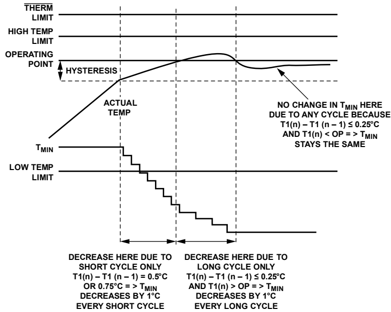
Figure 72. Effect of Exceeding Operating Point Minus Hysteresis Temperature
