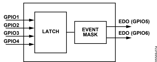
Figure 85. EDO Circuit
