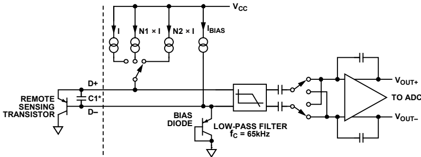
Figure 34. Input Signal Conditioning
