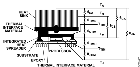
Figure 67. Thermal Model
