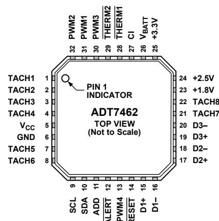
Figure 4. Configuration Option 1
