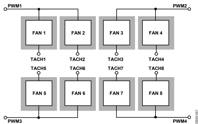
Figure 49. Synchronizing Fan PWM Output and TACH Inputs
