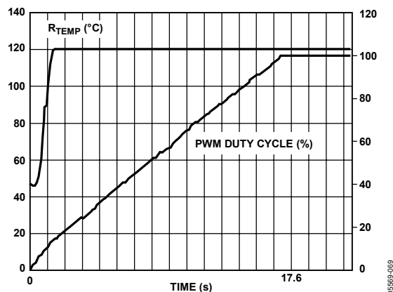
Figure 80. Enhanced Acoustics Mode with Ramp Rate = 2
