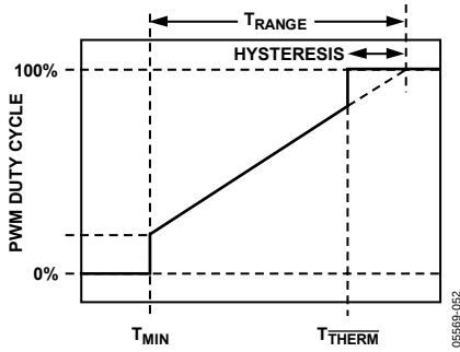
Figure 64. How T_{THERM} Relates to Automatic Fan Control
