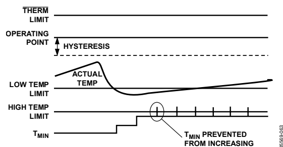
Figure 74. T_{MIN} Adjustments Limited by High Temperature Limit
