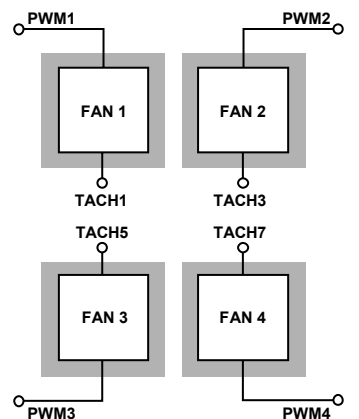
Figure 50. Driving and Measuring the Speed on a Single Fan
