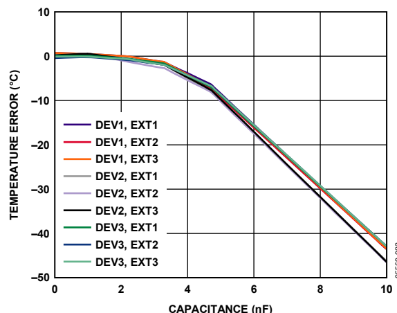
Figure 20. Remote Temperature Error vs. Capacitance Between D+ and D-
