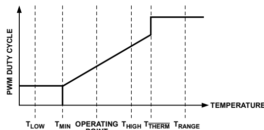
Figure 68. Dynamic T_{MIN} Control Loop
