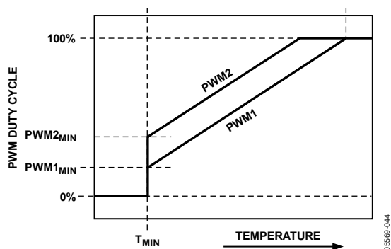
Figure 56. Operating Two Different Fans from a Single Temperature Channel
