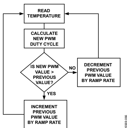
Figure 77. Enhanced Acoustics Mode Algorithm
