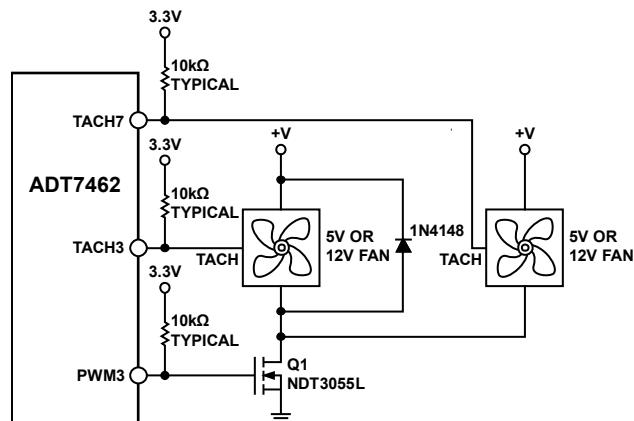
Figure 43. Interfacing Two Fans in Parallel to a PWM Output Using a Single N-Channel MOSFET
