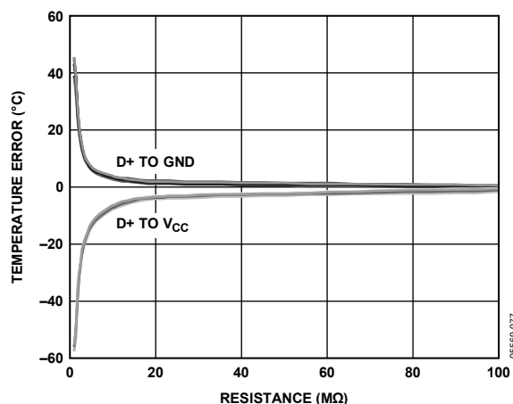
Figure 15. Remote Temperature Error vs. Resistance (SRC)
