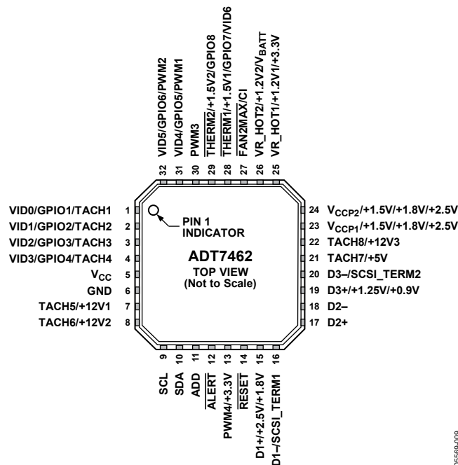
Figure 3. Pin Configuration
