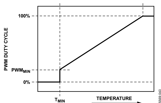
Figure 55. PWM MIN Determines Minimum PWM Duty Cycle at T MIN
