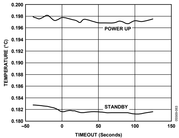
Figure 21. Local Temperature vs. Power-On Reset Timeout
