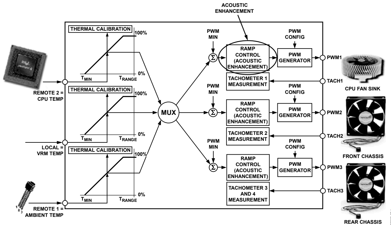
Figure 75. Acoustic Enhancement Smooths Fan Speed Variations Under Automatic Fan Speed Control
