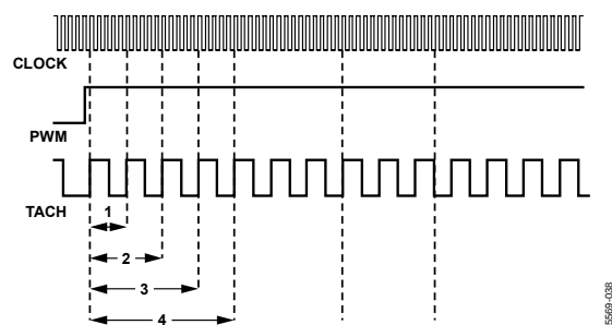
Figure 48. Fan Speed Measurement
