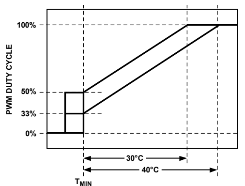
Figure 59. Adjusting PWM MIN Affects T RANGE
