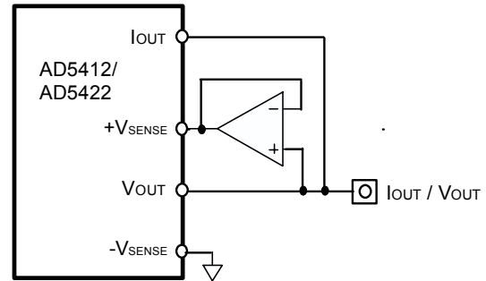
Figure 65. Connecting I_{\text{OUT}} and V_{\text{OUT}} to one connector
