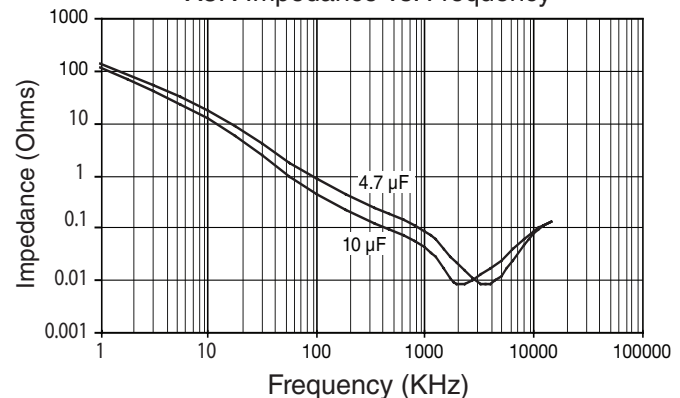
X5R Impedance vs. Frequency
