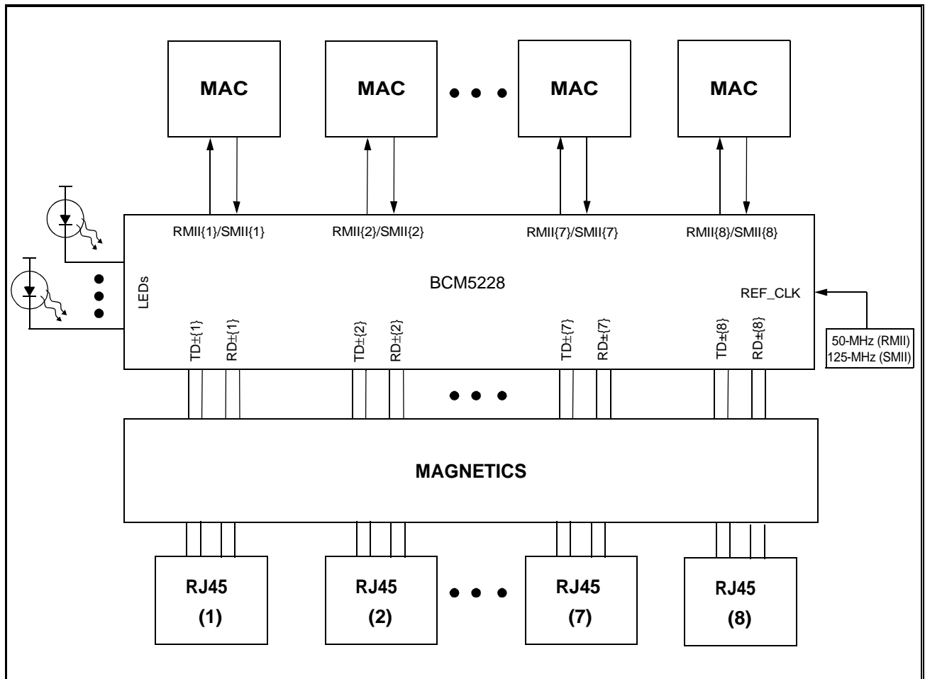
Figure 16: Switch Application
