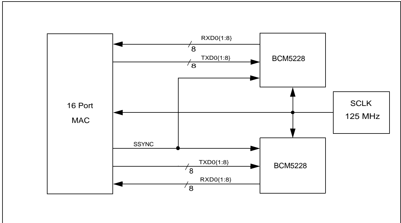
Figure 14: SMI Application
