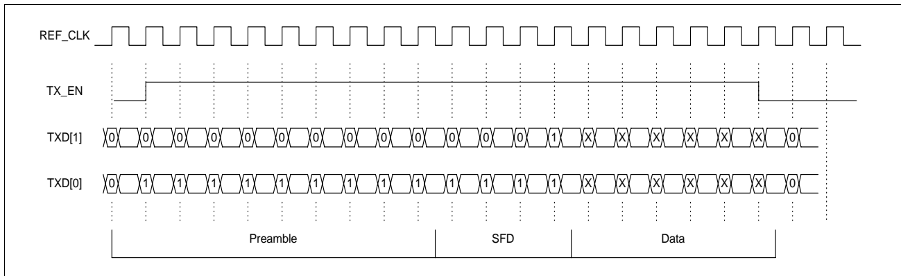
Figure 6: RMII Transmit Packet Timing
