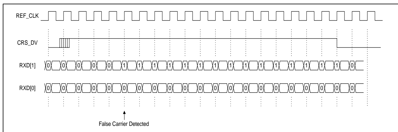
Figure 8: RMI Receive Packet with False Carrier
