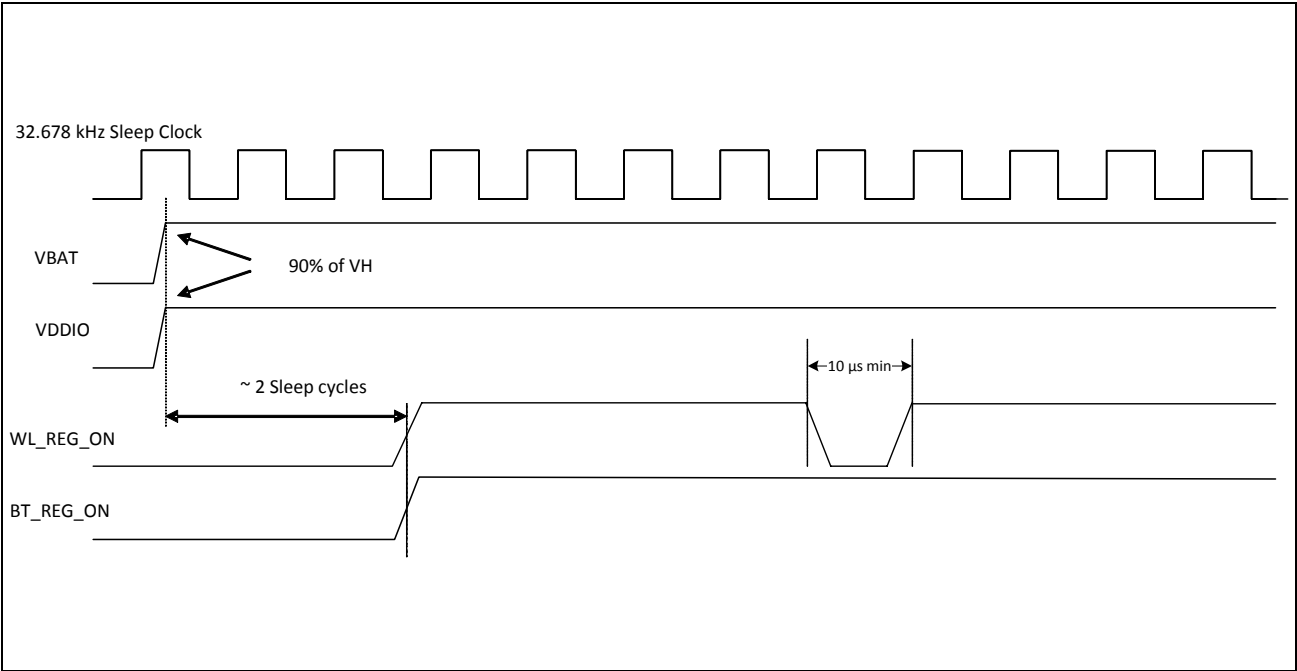
Figure 51: WLAN Warm Reset
