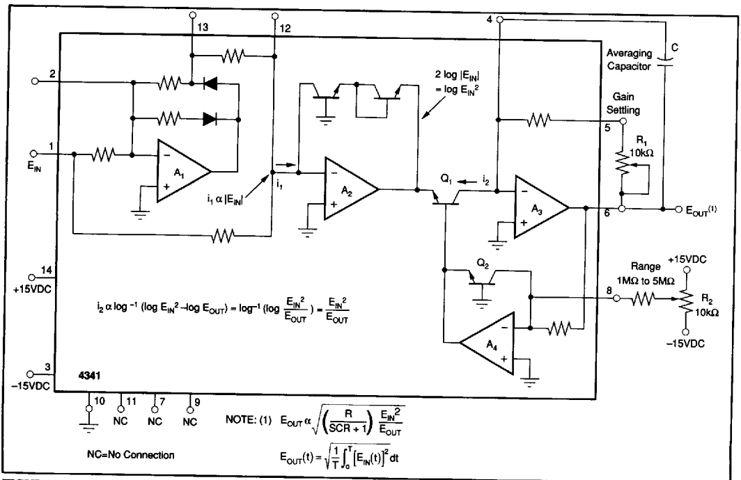
FIGURE 1. Simplified Schematic.
