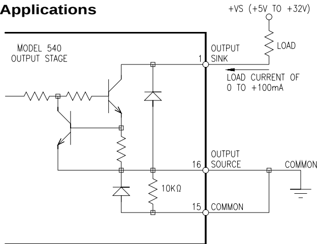
FIGURE 4. Model 540 Connected For Current-Sinking Mode
