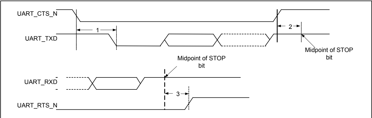
Figure 12: UART Timing
