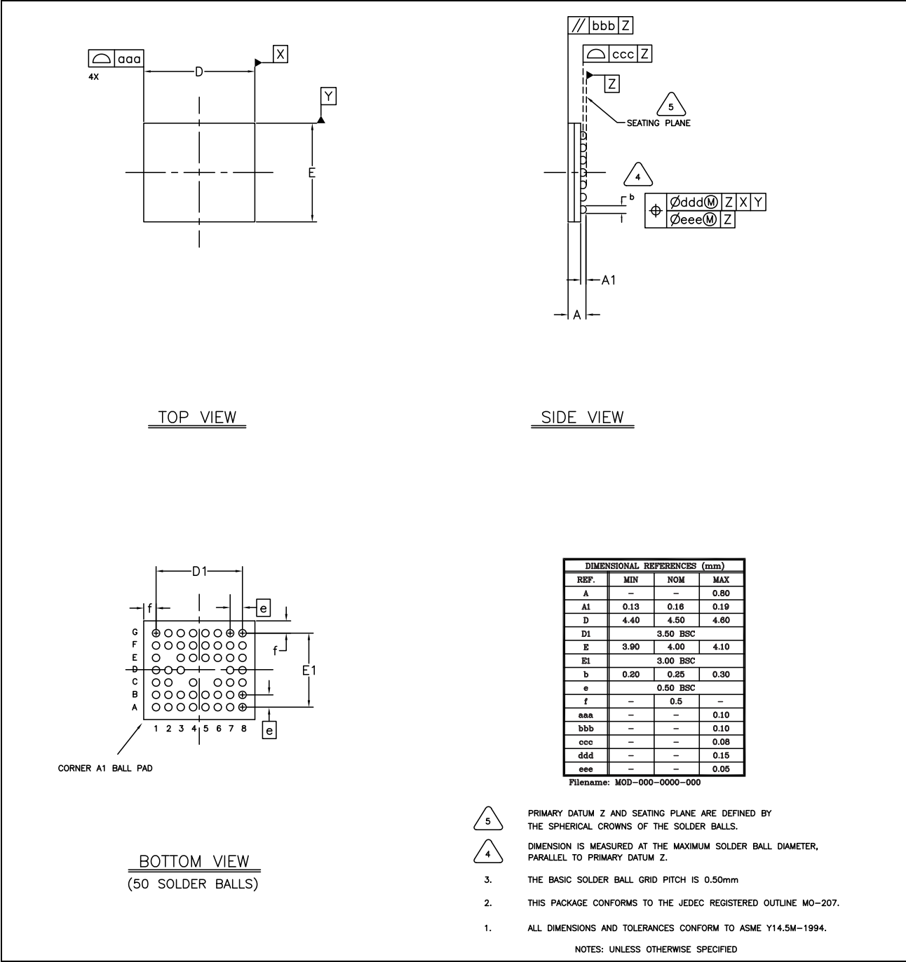
Figure 18: 50-Ball WFBGA Mechanical Drawing
