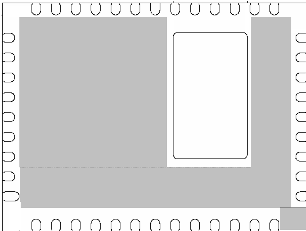
Figure 4. Lead-Frame exposed metal. Grey area highlights exposed metal that is not to be mechanically or electrically connected to the PCB.
