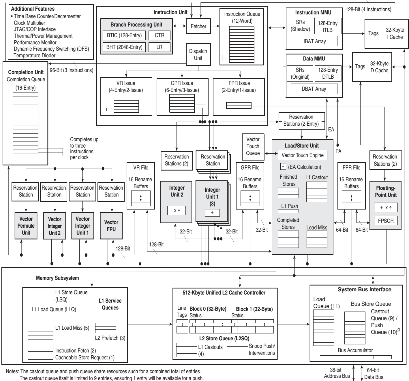
Figure 1-1. PC7447A Microprocessor Block Diagram
