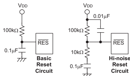
Reset Circuit
