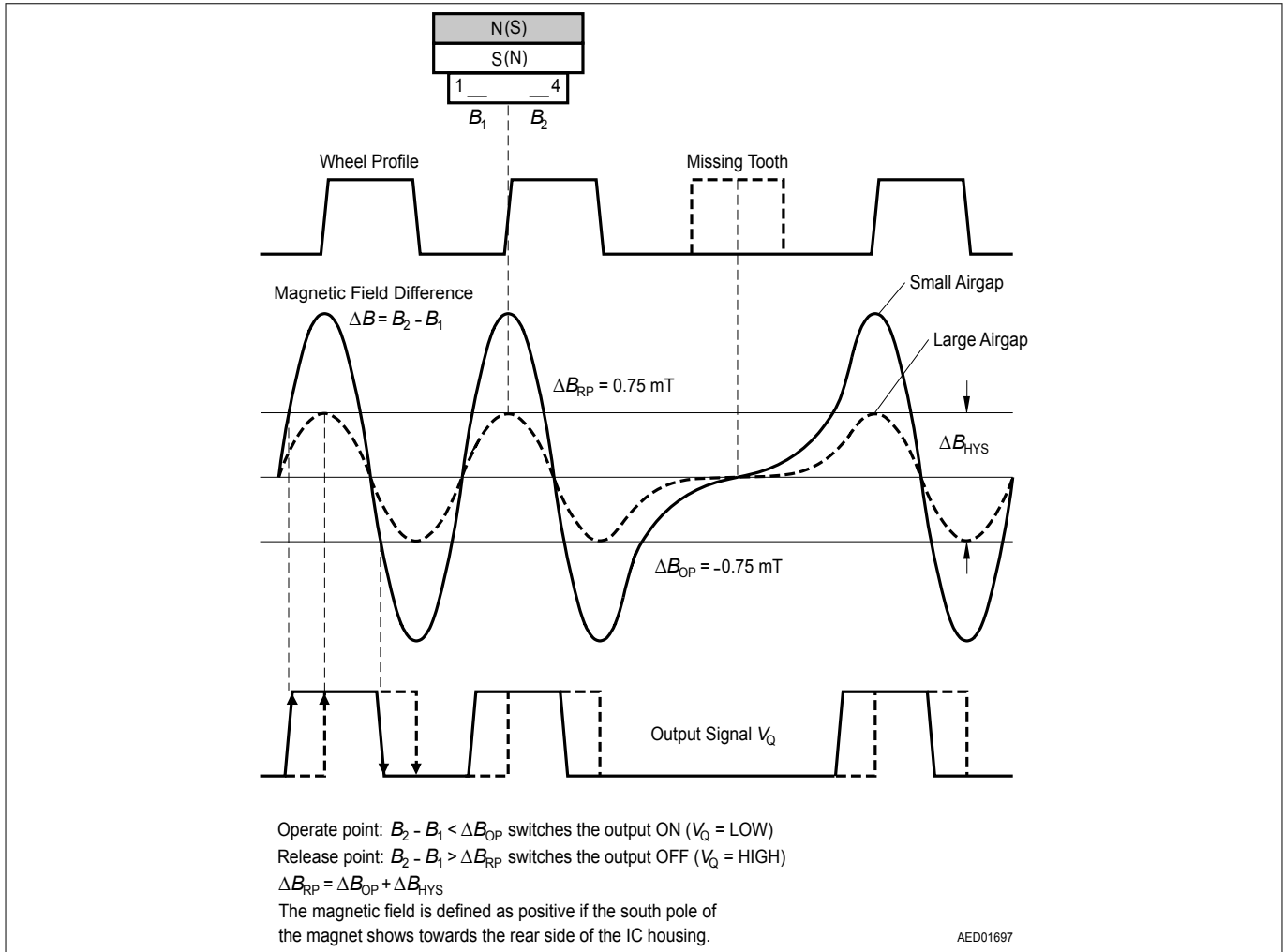
Figure 10 System Operation
