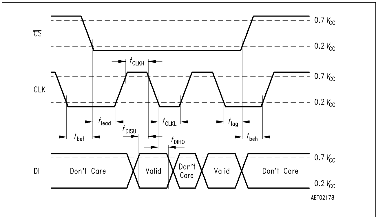
Figure 11 SPI-Input Timing
