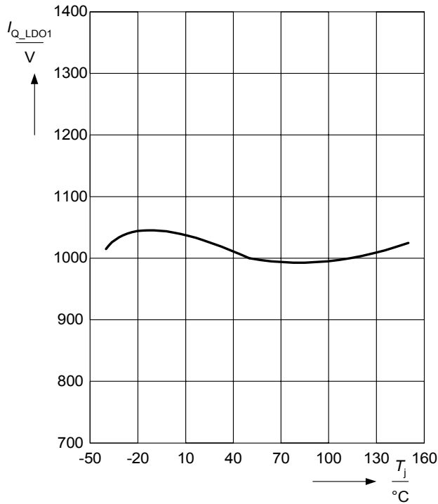
Q_LDO1 current limit vs. junction temperature
