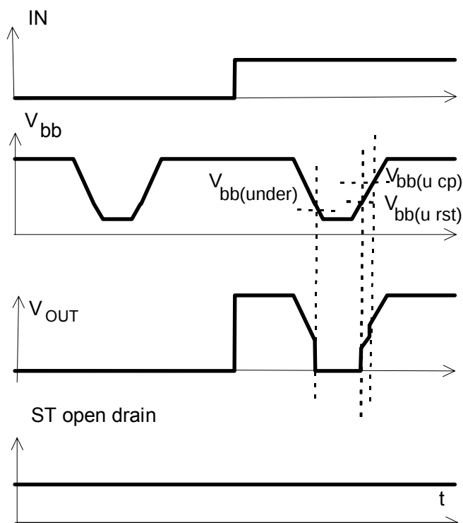
Figure 6a: Undervoltage:
