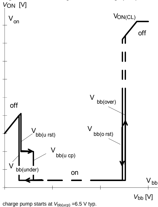
Figure 7a: Overvoltage:
