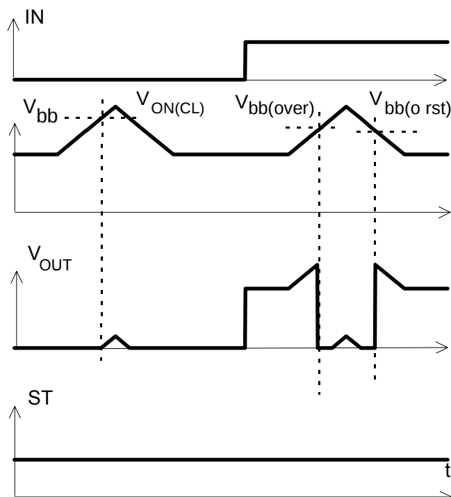
Figure 7a: Overvoltage:
