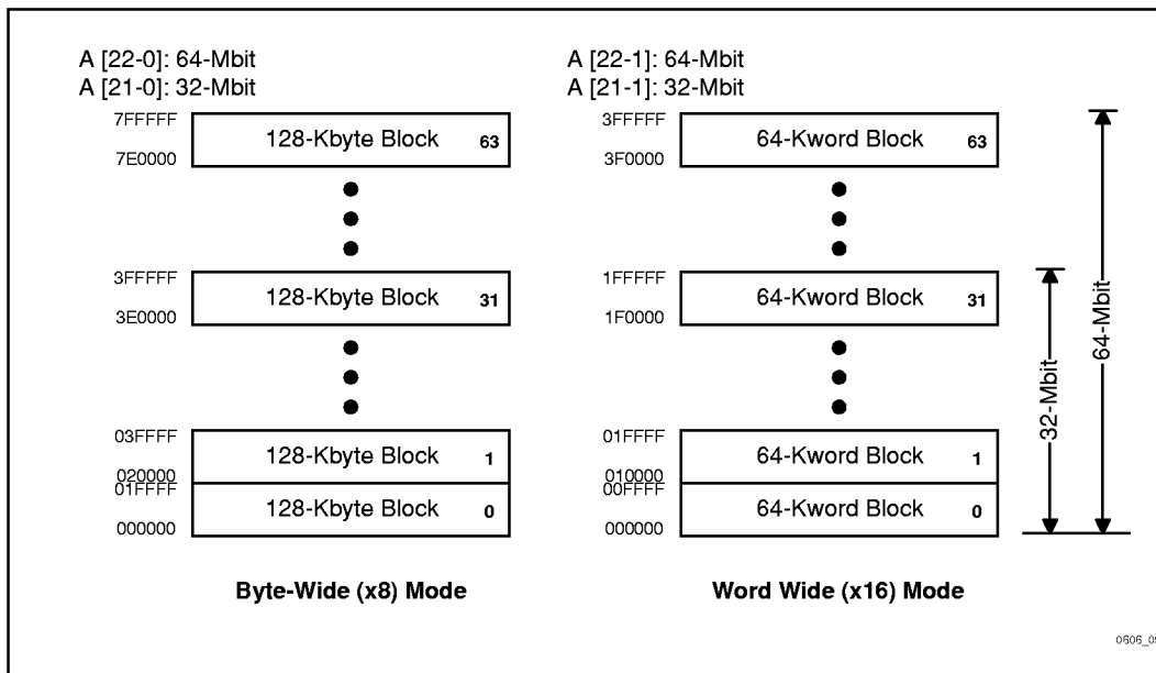
Figure 5. Memory Map
