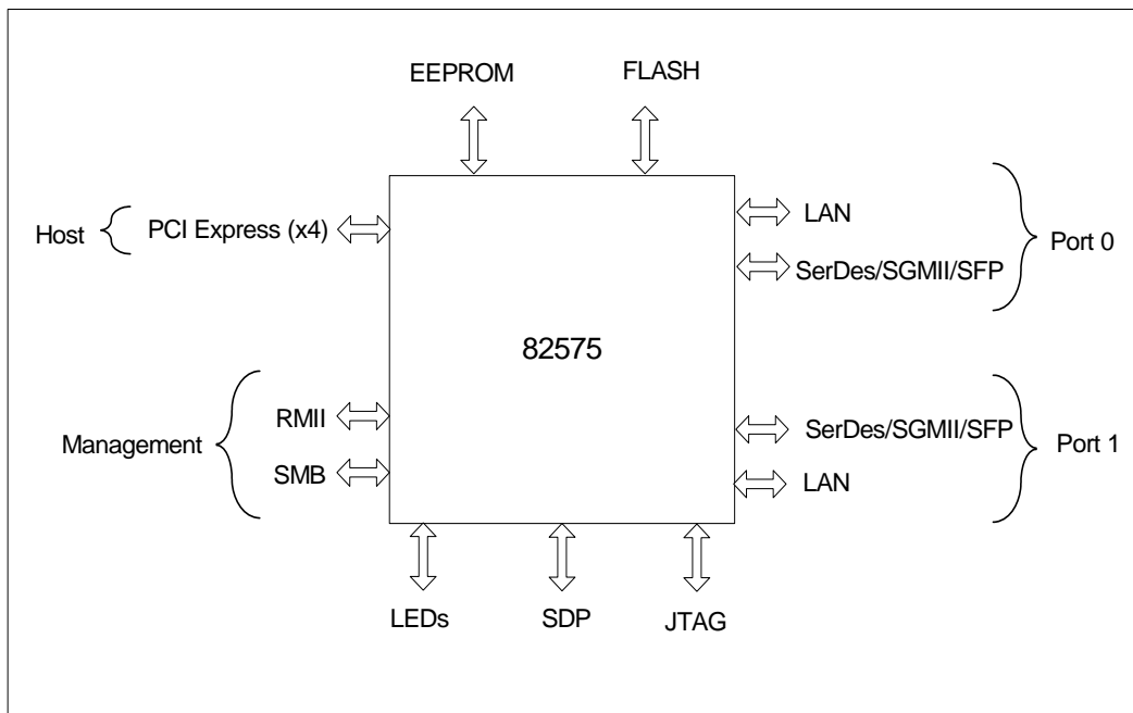
Figure 1. 82575EB Gigabit Ethernet Controller Block Diagram
