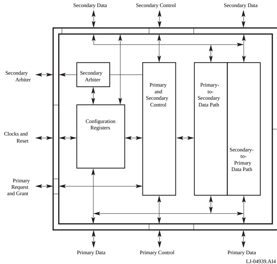
Figure 3. 21152 Block Diagram
