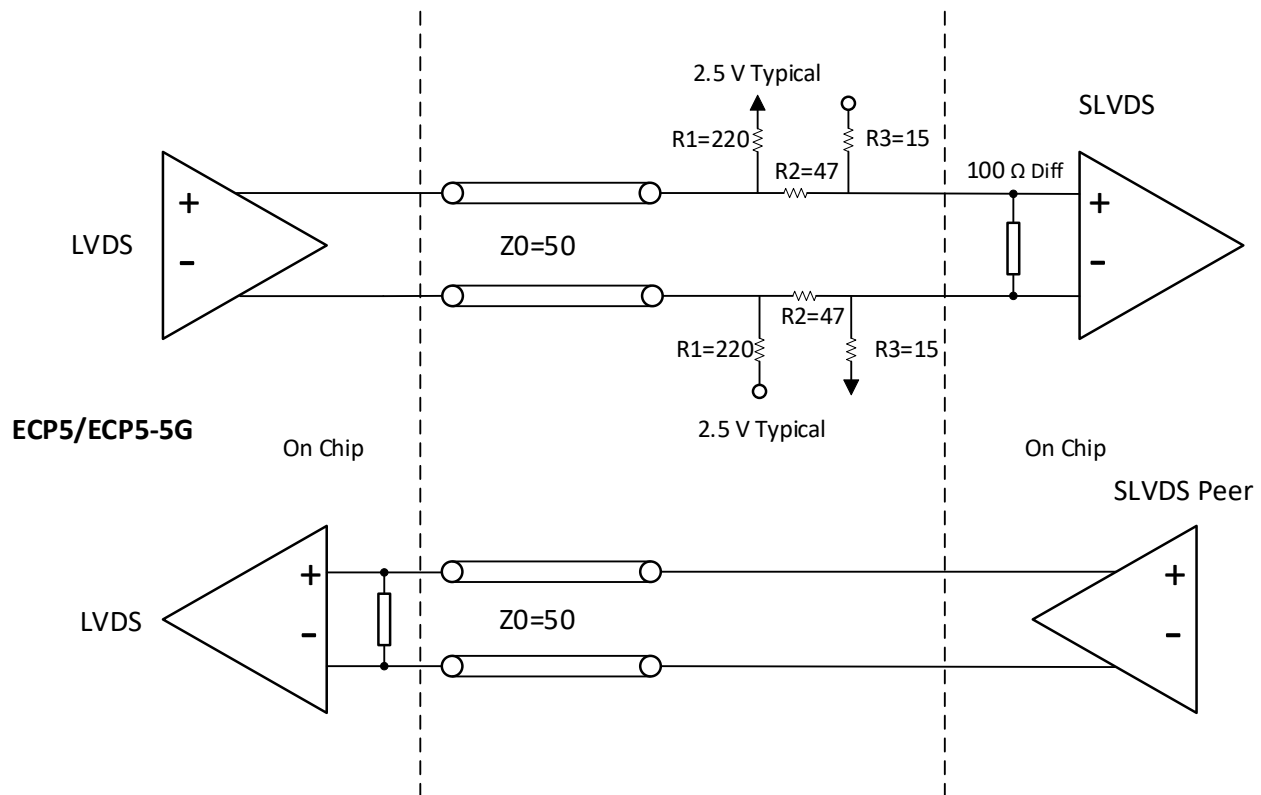
Figure 3.5. SLVS Interface
