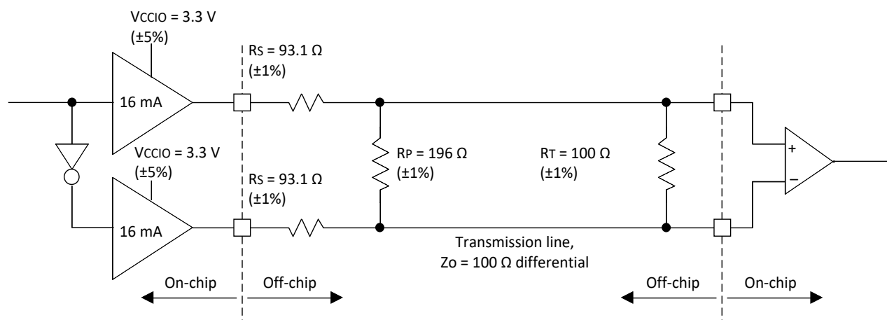
Figure 3.3. Differential LVPECL33
