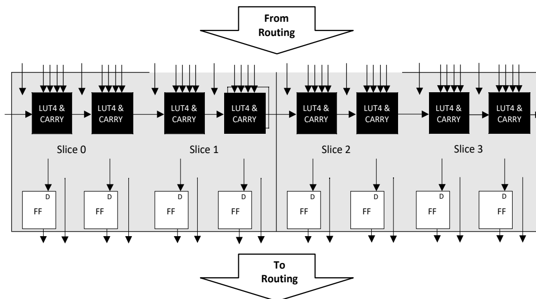
Figure 2.2. PFU Diagram
