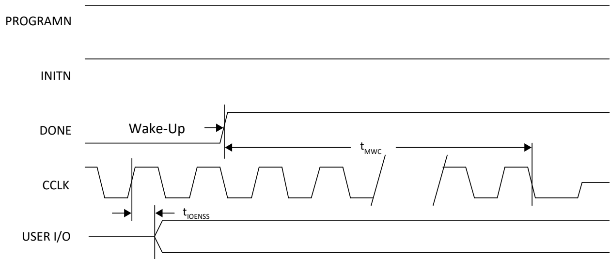
Figure 3.21. Wake-Up Timing
