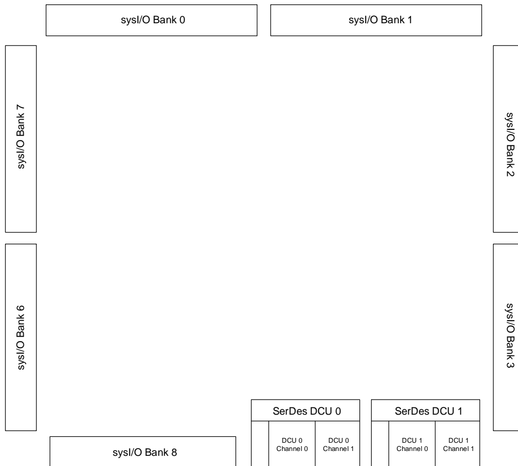
Figure 2.27. SerDes/PCS Duals (LAE5UM-45)
