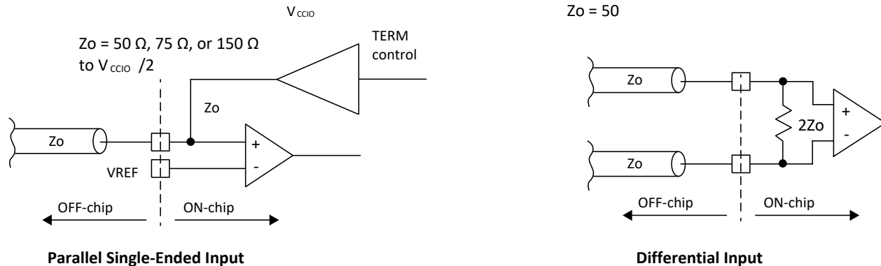
Figure 2.26. On-chip Termination
