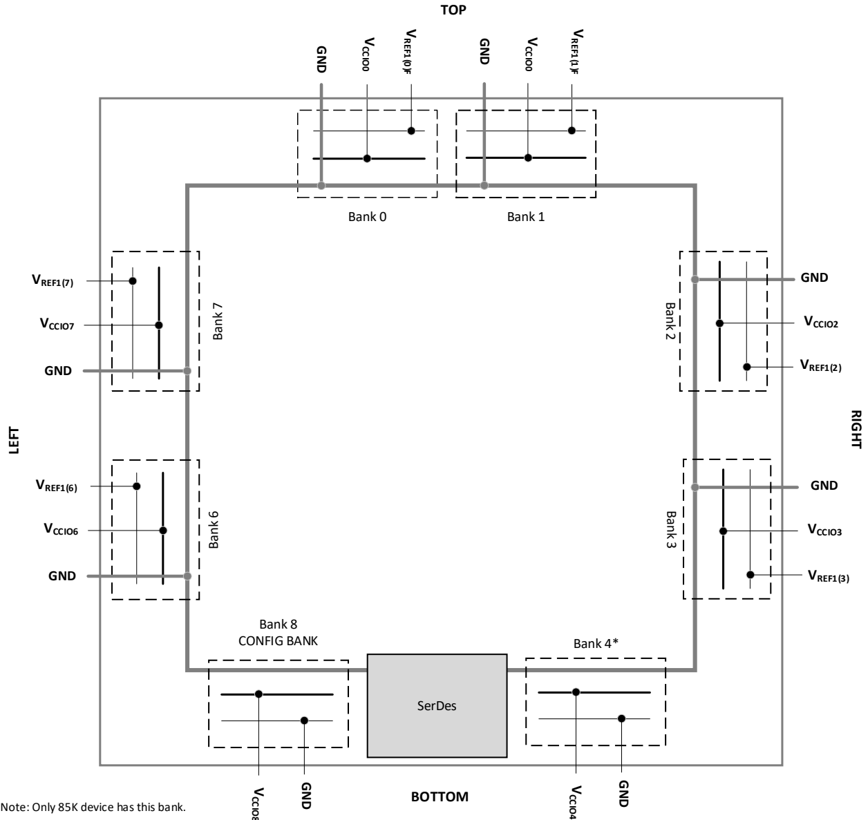
Figure 2.25. ECP5 Automotive Device Family Banks
