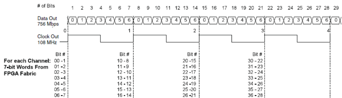
Figure 4.5. DDRX71, DDRX141 Video Timing Waveforms
