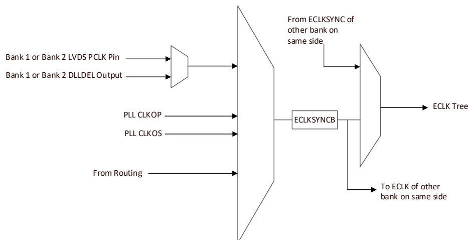
Figure 3.13. CrossLink Automotive Edge Clock Sources per Bank
