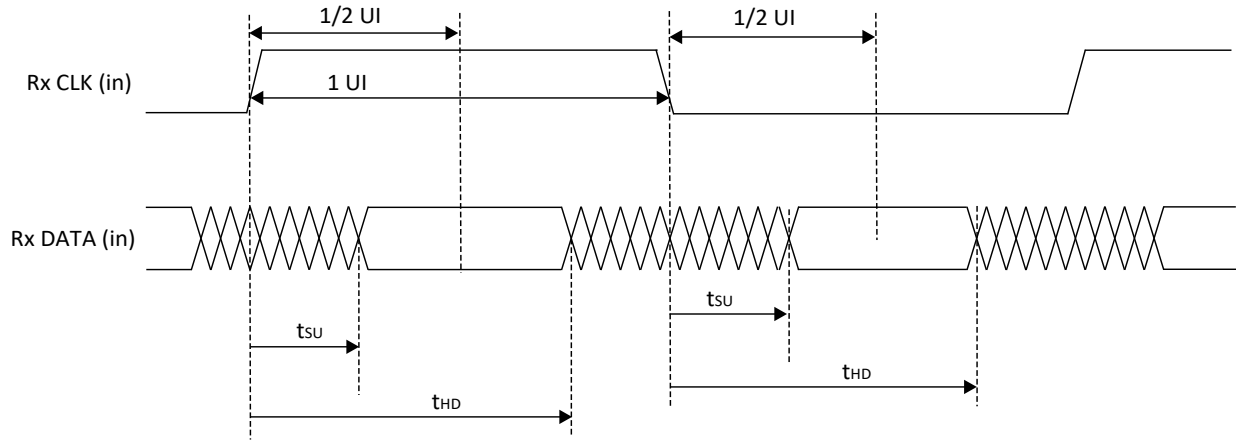
Figure 4.2. Receiver RX.CLK.Aligned Input Waveforms
