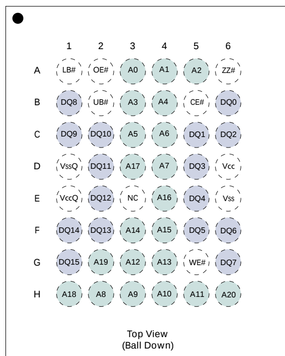
Figure 1: 48-Ball VFBGA Ball Assignment
