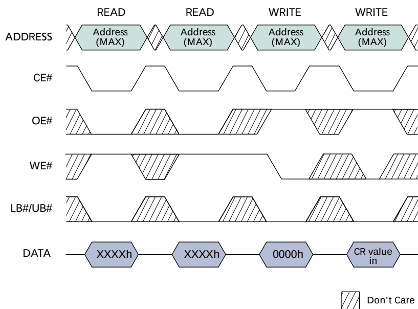
Figure 10: Software Access Load Configuration Register
