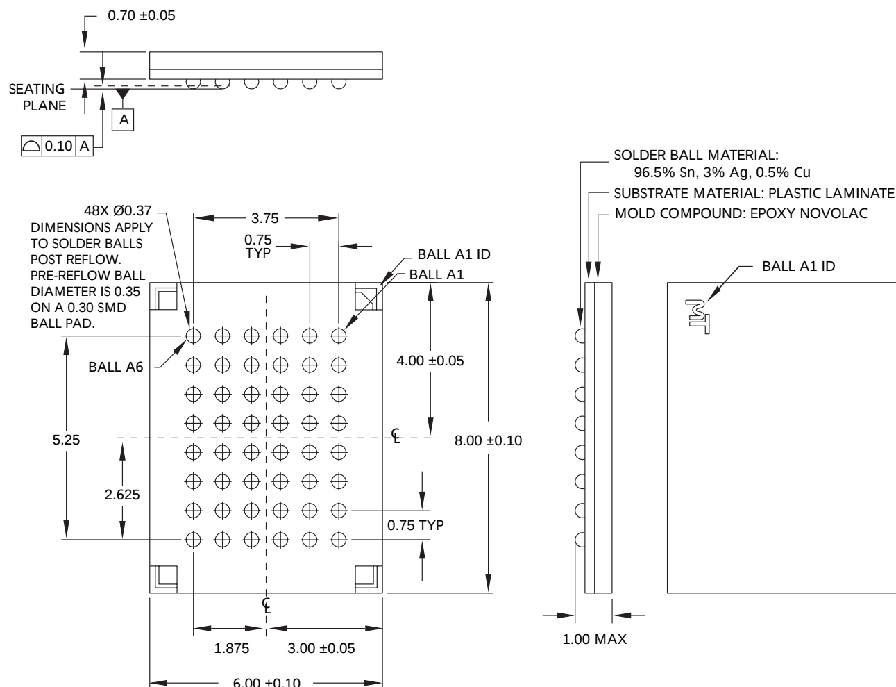
Figure 24: 48-Ball VFBGA
