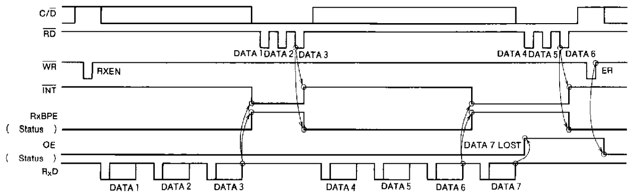
Receiver control and flag timing (block length=5)
