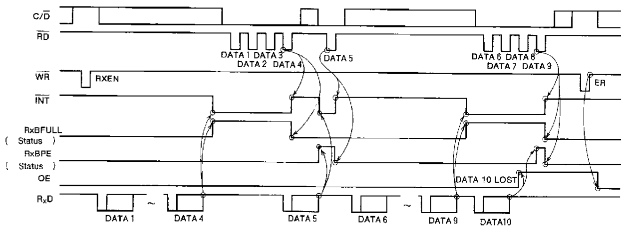
Receiver control and flag timing (block length=5)
