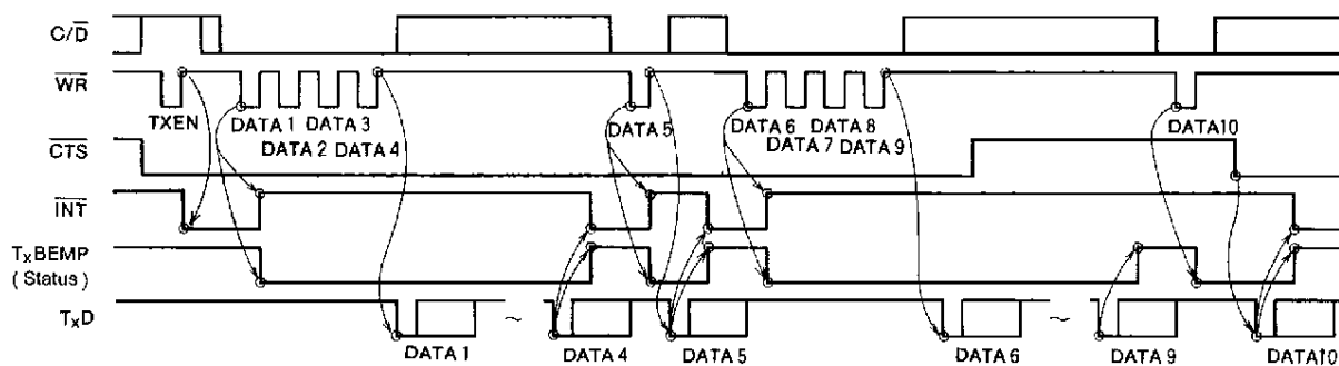
Transmitter control and flag timing (block length=5)
