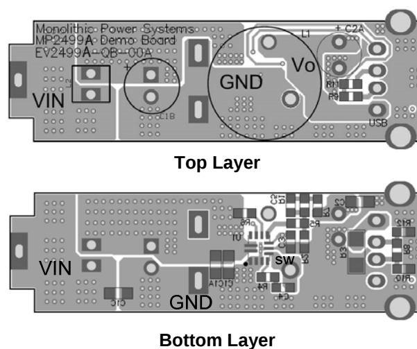
Figure 9: Recommended Layout
