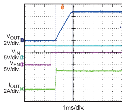
Start-Up through Enable CC Load = 3A
