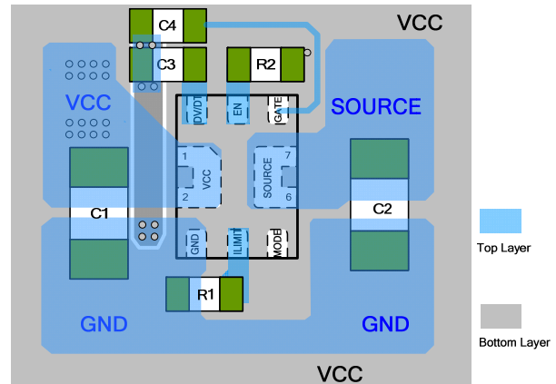
Figure 4: Recommended Layout
