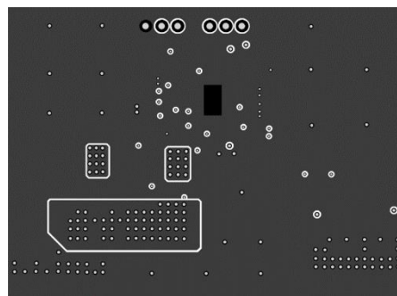
Mid-Layer 1
