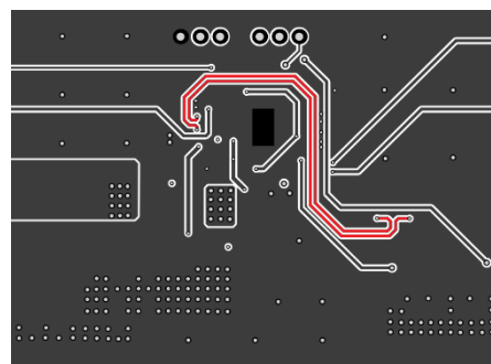
Mid-Layer 2
