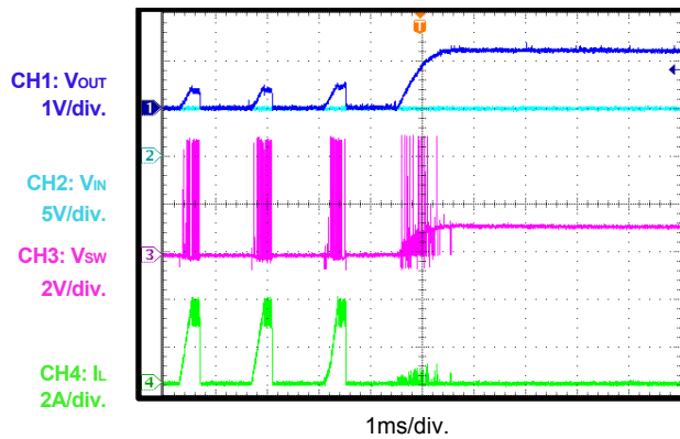
Short-Circuit Recovery
