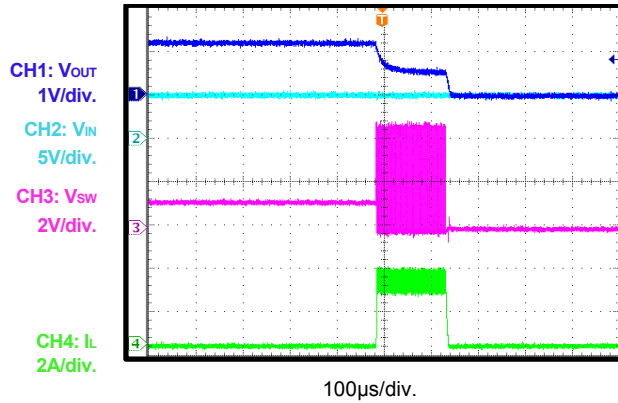
Short-Circuit Recovery
