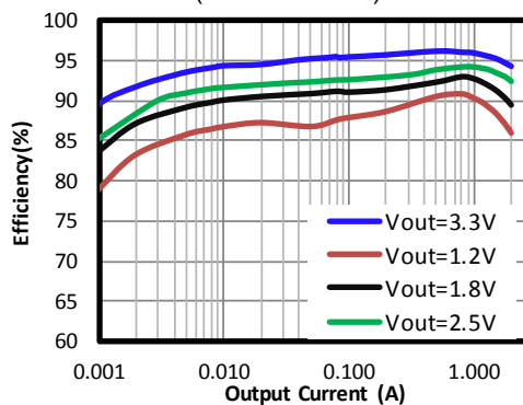
Efficiency vs. Output Current V IN = 5V(DCR=27mohm)
