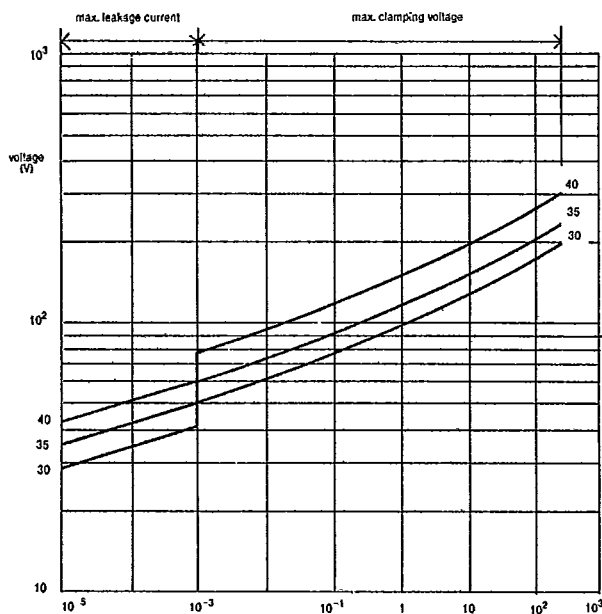
Fig. 11 V-I characteristics, 593 series, 30 to 40 V
