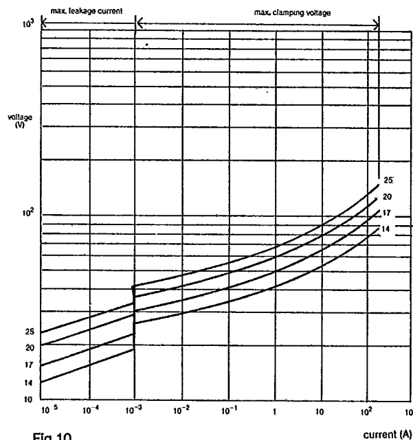
Fig. 10 V-I characteristics, 593 series, 14 to 25 V
