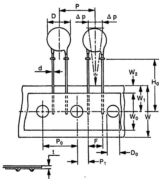
Fig. 33C Flanged Lead
