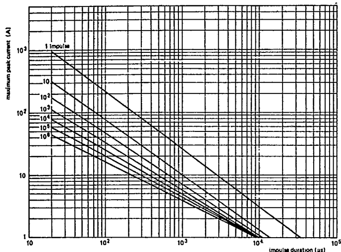
Fig. 27 Max. applicable transient current as a function of impulse duration, 595 series, 14 to 40 V
