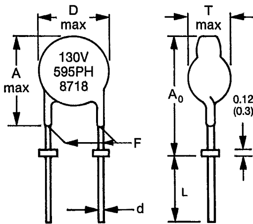
Figure 32C Flanged Lead
