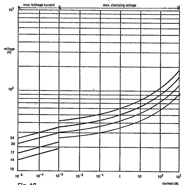
Fig. 16 V-I characteristics, 595 series, 14 to 25 V
