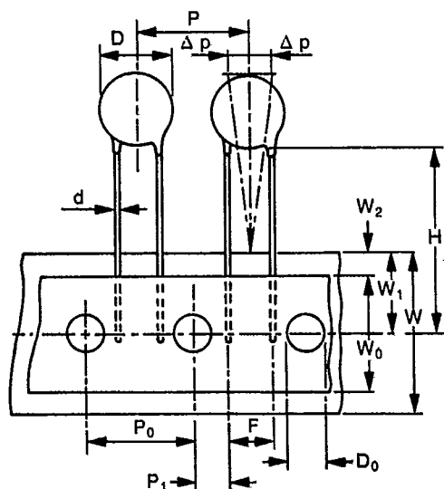
Fig. 33 Straight Lead
