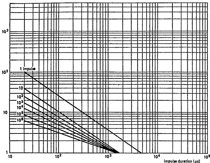
Fig. 21 Max. applicable transient current as a function of impulse duration, 592 series, 14 to 40 V
