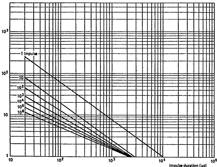
Fig. 23 Max. applicable transient current as a function of impulse duration, 593 series, 14 to 40 V
