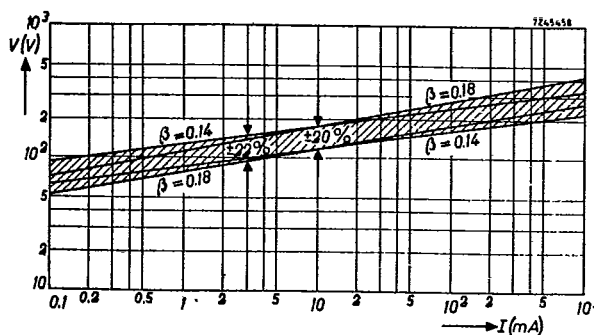
Fig. 5 Spread of voltage/current characteristic due to \beta -tolerance.
