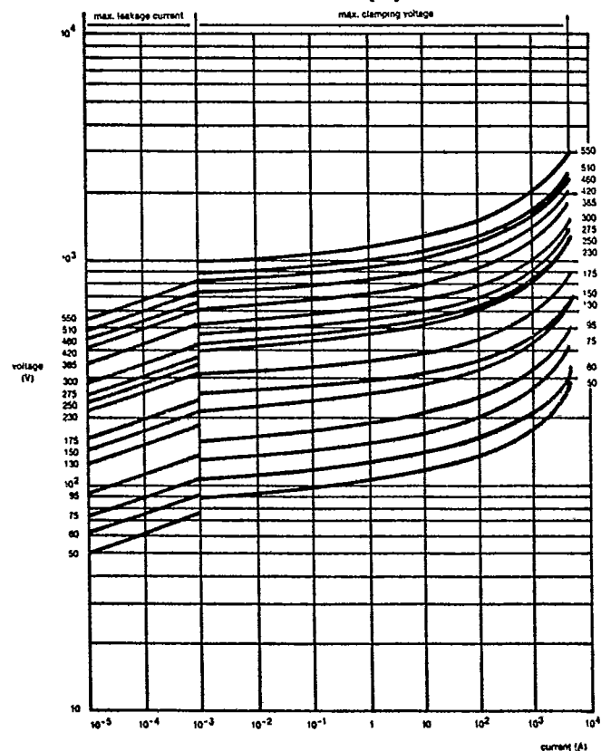
Fig. 20 V-I characteristics, 596 series, 50 to 550 V
