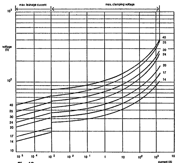
Fig. 19 V-I characteristics, 596 series, 14 to 40 V
