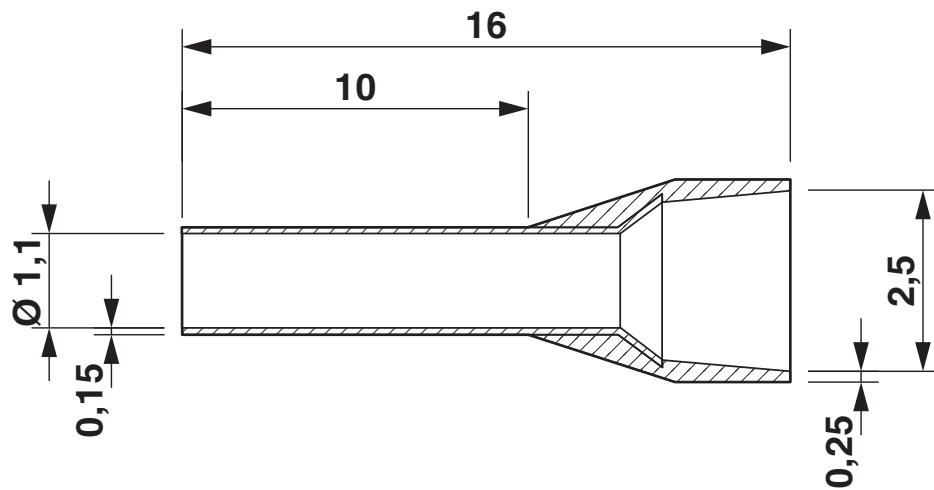
Dimensional drawing
