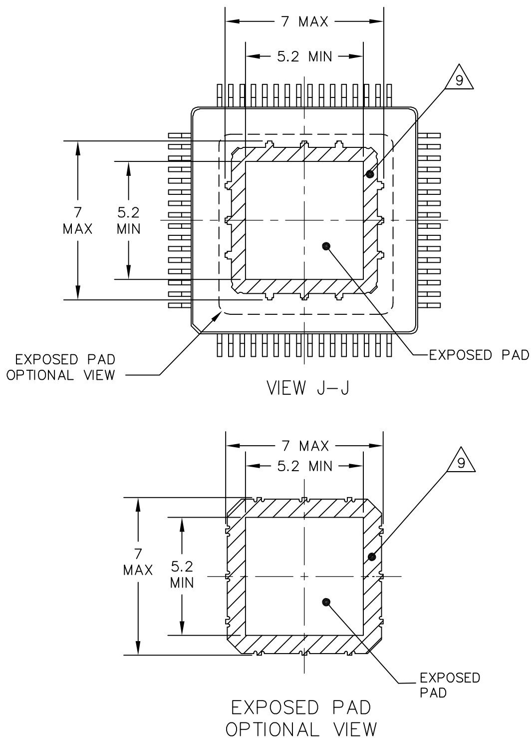
Figure K-2. 64 LQFP Exposed Pad Package
