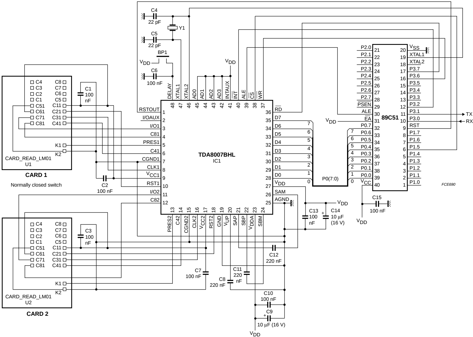
Fig.16 Application diagram.
