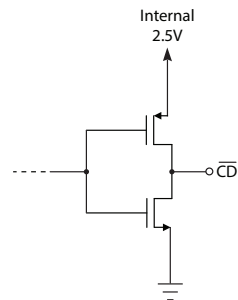
Figure 3-5: \overline{CD} Circuit
