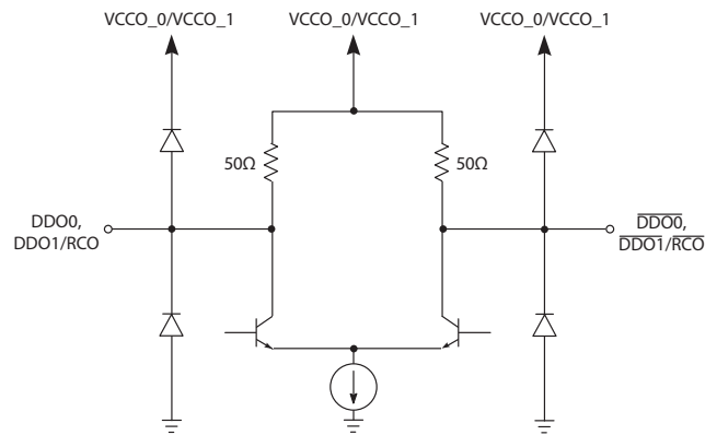
Figure 3-2: DDO0, \overline{\text{DDO0}} , DDO1/RCO, \overline{\text{DDO1}}</math>/RCO Serial Data Output
