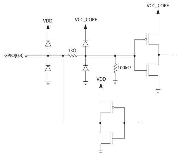
Figure 3-6: GPIO[0:3]
