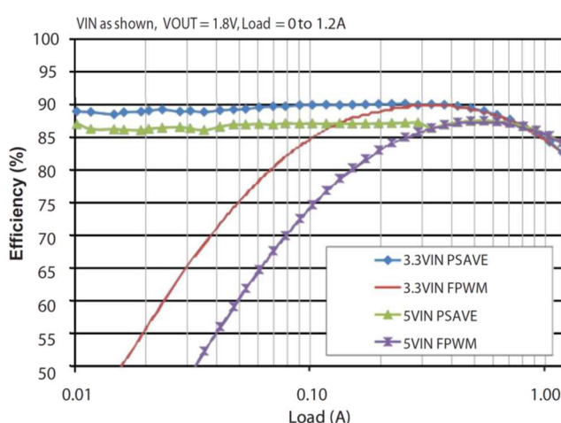
Efficiency vs. Load - VOUT 1.8V
