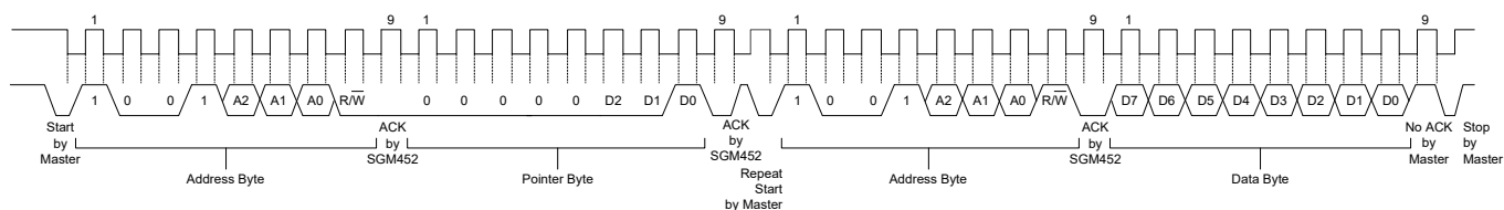
(a) Typical Pointer Set Followed by Immediate Read from Configuration Register
