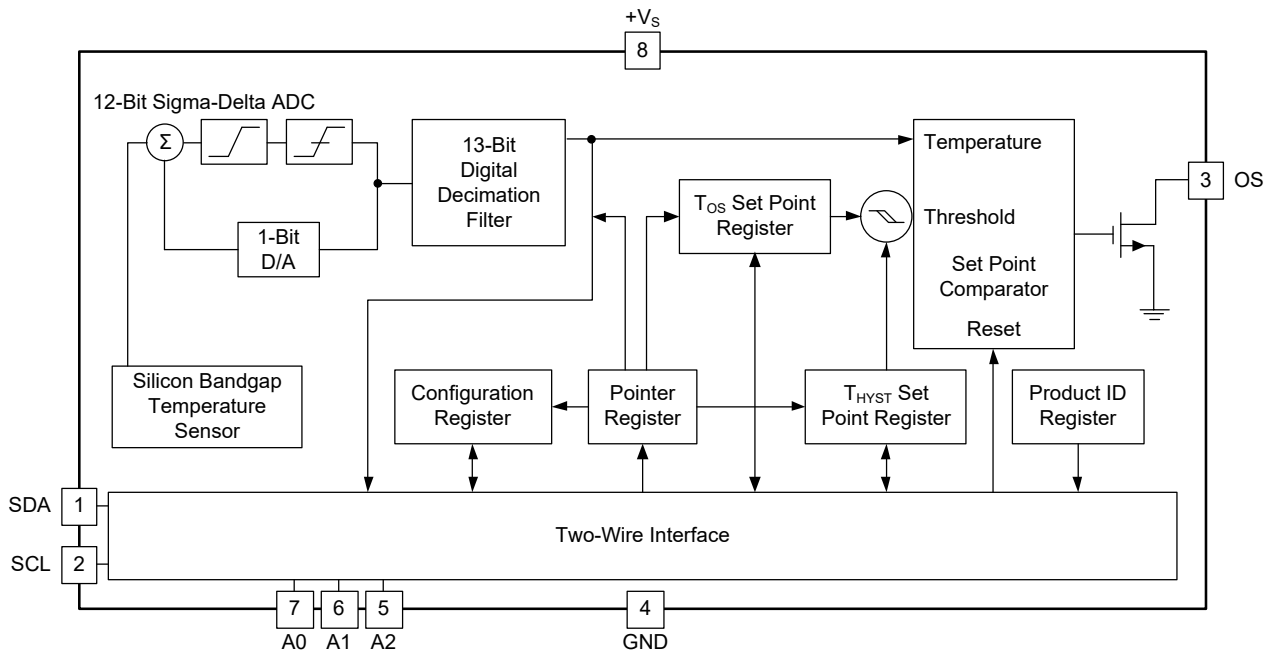
Figure 5. Block Diagram
