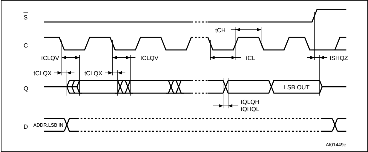
Figure 29. Output timing
