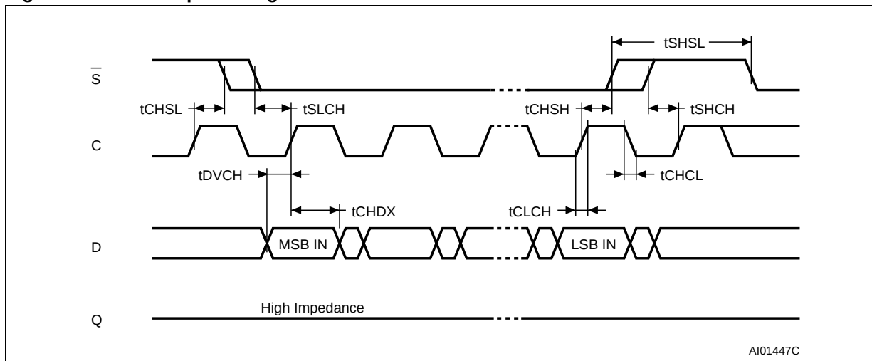
Figure 27. Serial input timing
