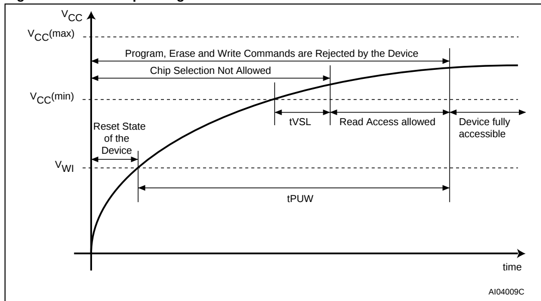
Figure 25. Power-up timing
